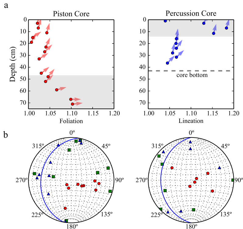
Fig. 3. AMS fabric in the piston core (left column) and percussion core (right column). a) Plots showing the variation in lineation ( L = k_{\max}/k_{\min} ) and foliation ( F = k_{\text{int}}/k_{\min} ) versus depth in the piston and percussion cores respectively. Vectors represent the magnitude and inclination of the k_{\min} principle susceptibility axis. b) Maximum (squares), intermediate (triangles), and minimum (circles) principal susceptibilities with disturbed sections omitted to highlight the natural fabric. k_{\max} orientations trend towards a shallow plane depicted by the blue line. As the cores are not azimuthally oriented, the three principal susceptibility axes have been rotated by a constant so that the k_{\min} axes plunge eastward or 'down-glacier', consistent with experimental observations from sheared diamict (Hooyer et al., 2008). (For interpretation of the references to color in this figure legend, the reader is referred to the web version of this article.)
