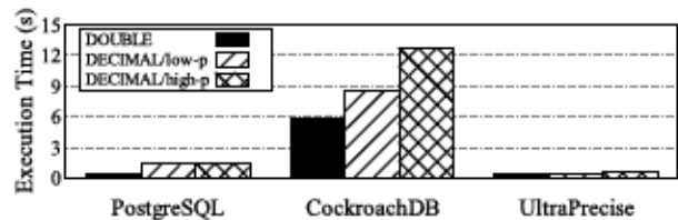
Fig. 1. Execute SELECT SUM(c1+c2) FROM R in PostgreSQL, CockroachDB, and UltraPrecise. R has 10 million tuples. c1 and c2 are set to (1) both DOUBLE, (2) DECIMAL(17, 5) and DECIMAL(14, 2), namely low-p , and (3) DECIMAL(35, 5) and DECIMAL(32, 2), namely high-p .
