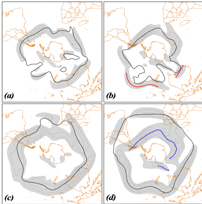
Figure 2. (a) Isotachs of the daily averaged wind speed (contoured every 10 m s -1 and shaded above 30 m s -1 ) and the core isertel (bold black line) in the 310:325 K isentropic layer on 13 July 1995 from the JRA-55 reanalysis data. The core isertel value is -1.3 PVU. (b) As in (a) but for 24 August 2001. Core isertel value is -2.0 PVU. Dashed red line indicates a portion of the core isertel from the overlying STJ layer (depicted in Fig. 2d). (c) As in (a) but for wind speeds and the core isertel in the 340:355 K isentropic layer on 13 July 1995. Core isertel value is -3.6 PVU. (d) As in (c) but for 24 August 2001. Core isertel value is -1.4 PVU. Dashed blue line indicates a portion of the core isertel from the underlying POLJ layer (depicted in Fig. 2b). See the text for further explanation.
