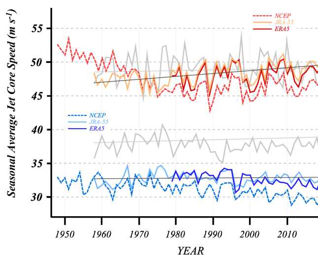
Figure 7. Seasonal-average U along the core isertel for the subtropical (red lines) and polar (blue lines) jets from each of the three SH reanalysis data sets. The thin black lines are trend lines for each time series from the JRA-55 data. Gray lines are the equivalent boreal-winter U analysis from Fig. 9 of Martin (2021).
