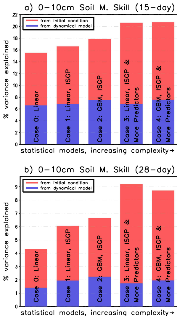
FIG. 5. As in Fig. 4, but for forecasts of the future anomaly of shallow (0–10 cm) soil moisture.
