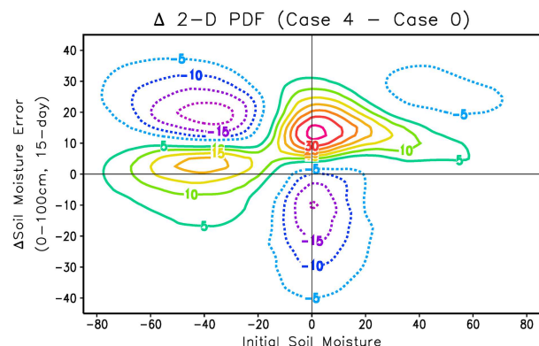
FIG. 10. As in Fig. 9, but for the two-dimensional PDF as a function of initial 0–100-cm soil moisture ( x axis; \text{kg m}^{-2} ) and the error in the 15-day 0–100-cm soil moisture forecast ( y axis; \text{kg m}^{-2} ). The PDF is multiplied by 1 \times 10^6 prior to plotting.
