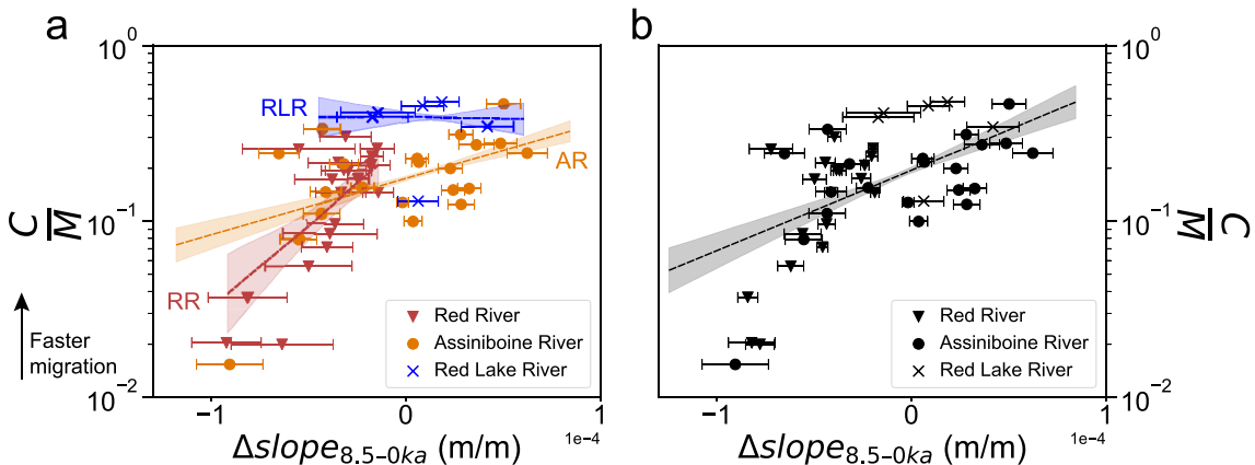
Figure 3. (a) Regressions of \Delta \text{slope}_{8.5-0\text{ka}} and \log of normalized cutoff count ( \frac{C}{M} ) for the Red River (red), Assiniboine River (orange), and Red Lake River (blue). Shaded regions show 95% confidence interval for Monte Carlo ensemble. Dashed lines show median regression. (b) Regression of \Delta \text{slope}_{8.5-0\text{ka}} and \log of normalized cutoff count ( \frac{C}{M} ) for all three rivers as a single analysis. Dashed line shows median regression.
