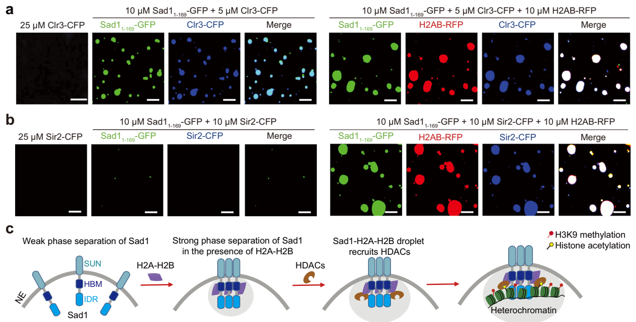
Fig. 7 | H2AB-enhanced phase separation of Sad1 facilitates HDAC recruitment. a Fluorescence images of Clr3-CFP alone, Sad1 1-169 -GFP mixed with Clr3-CFP, and a mixture containing Sad1 1-169 -GFP, H2AB-RFP, and Clr3-CFP. Clr3-CFP alone could not form liquid-like droplets, but could be incorporated into the same Sad1 droplets and Sad1-H2AB droplets. Scale bars, 10 \mu\text{m} . b Fluorescence images of Sir2-CFP alone, Sad1 1-169 -GFP mixed with Sir2-CFP, and a mixture containing Sad1 1-169 -GFP, H2AB-RFP, and Sir2-CFP. Sir2-CFP alone could not form liquid-like droplets. Sir2-
