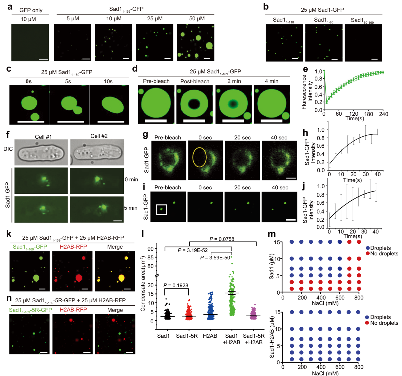
Fig. 6 | H2A-H2B promotes Sad1 phase separation. a Fluorescence microscopy images of the Sad1 1-169 -GFP fusion protein at different concentrations in droplet formation buffer containing 150 mM NaCl and 10% PEG-8000. Scale bars, 10 \mu m. GFP serves as the negative controls and shows no LLPS at the tested concentration. b Fluorescence images of different Sad1 constructs in the droplet formation buffer. Scale bars, 10 \mu m. c Fluorescence images of the same view field showing the dynamic fusion of the Sad1 droplets. Scale bars, 10 \mu m. d Fluorescence images of Sad1 1-169 -GFP before and after photobleaching. Scale bars, 10 \mu m. e Quantitation of the normalized fluorescence recovery of Sad1 1-169 -GFP following droplet photobleaching. Data are presented as mean \pm SEM from n = 3 independent experiments. Source data are provided as a Source Data file. f Sad1 exhibits dynamic movement on the nuclear envelope. Time-lapse fluorescence microscopy of Sad1-GFP under its native promoter in WT cells. Scale bar, 2 \mu m. g Fluorescence images of mildly overexpressed Sad1-GFP during a FRAP experiment. The bleached region is indicated with a yellow oval. Scale bars, 1 \mu m. h The plot of normalized recovery of the overexpressed Sad1-GFP signal after photobleaching. Data are presented as mean \pm SD from n = 3 independent experiments. Source data are provided as a
