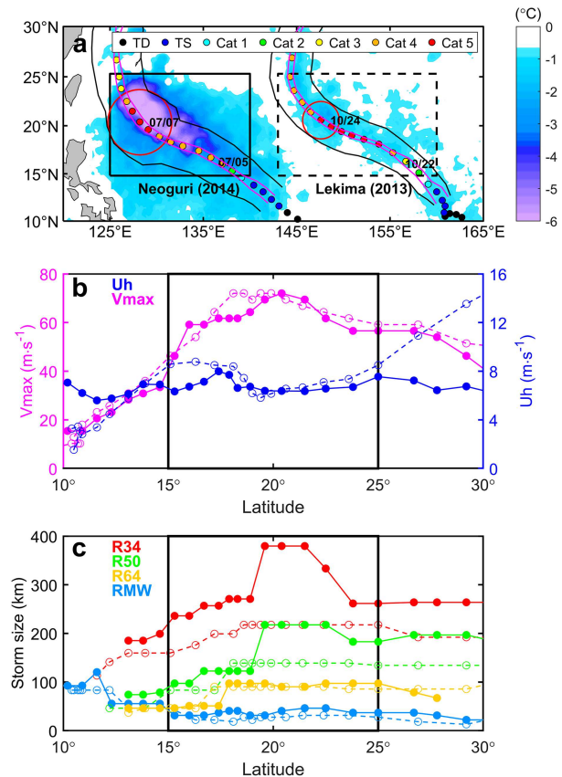
FIG. 2. Comparison of the cold wakes induced by a large versus a small TC. (a) Best tracks of TCs Neoguri (2014) (colored dots; leftward) and Lekima (2013) (colored dots; rightward), and the maximum SSTA left by the two TCs (background color), which is calculated with the minimum SST on days 0–5 post-TC minus pre-TC SST. The two TCs have nearly parallel tracks with a distance of about 2000 km, initially moving northwestward between 10^\circ and 25^\circ\text{N} and then turning to northward poleward of 25^\circ\text{N} . Coincidentally, both TCs reached their lifetime peak intensity with the same V_{\max} of 72 \text{ m s}^{-1} at around 20^\circ\text{N} . The black and magenta solid curves along TC tracks indicate the R34 and RMW of TCs, respectively. Red cycles show the R34 (380 and 218 km for Neoguri and Lekima, respectively) when the TC centers are located around 20^\circ\text{N} . The solid boxes indicate the focused domains. (b) TC intensity V_{\max} (magenta) and translation speed U_h (blue) as a function of latitude for TCs Neoguri (solid curve with closed circles) and Lekima (dashed curve with open circles). (c) As in (b), but for storm sizes represented by RMW (blue), R64 (yellow), R50 (green), and R34 (red). The focused domains from 15^\circ to 25^\circ\text{N} are indicated in (b) and (c) by black solid lines.
