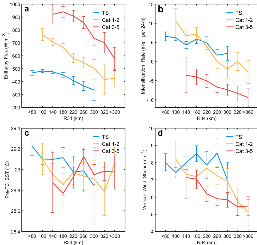
FIG. 10. Composited (a) enthalpy flux from ocean to TCs, (b) subsequent 24-h TC IR, (c) pre-TC SST averaged within 100 km of TC center, and (d) the vertical wind shear averaged within a ring of 200–800 km from TC center, as a function of R34 for TS (blue), Cat 1–2 (yellow), and 3–5 TCs (red). The vertical bars indicate error bars with 95% confidence intervals.
