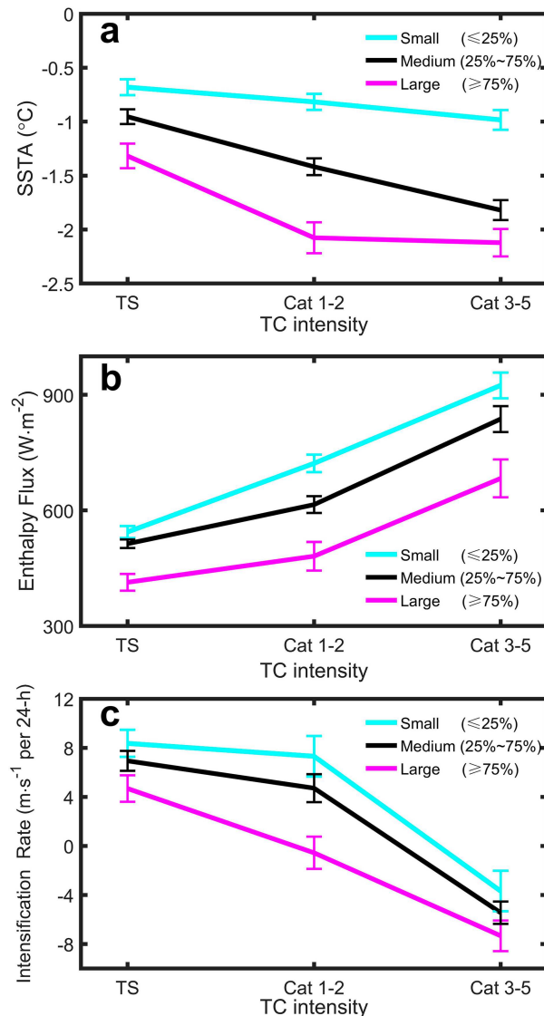
FIG. 11. Comparison of the (a) SSTA, (b) enthalpy flux, and (c) IR for groups with small ( R_{34} smaller than its 25th percentile; cyan), medium ( R_{34} between 25th and 75th percentiles; black), and large ( R_{34} larger than 75th percentile; magenta) for TS, Cat 1–2, and 3–5 TCs.
