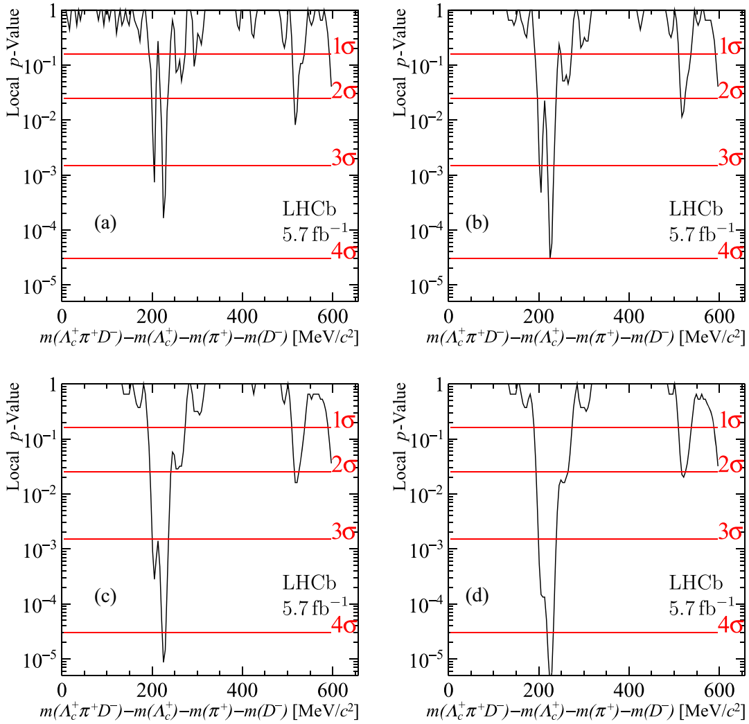
FIG. 4. Local p -value distributions for the \Lambda_c^+ \pi^+ D^- mode with different signal models: (a) Gaussian function, (b) Voigtian function with 5 \text{MeV}/c^2 width, (c) Voigtian function with 10 \text{MeV}/c^2 width, and (d) Voigtian function with 15 \text{MeV}/c^2 width. The red lines correspond to the levels of local significance.
