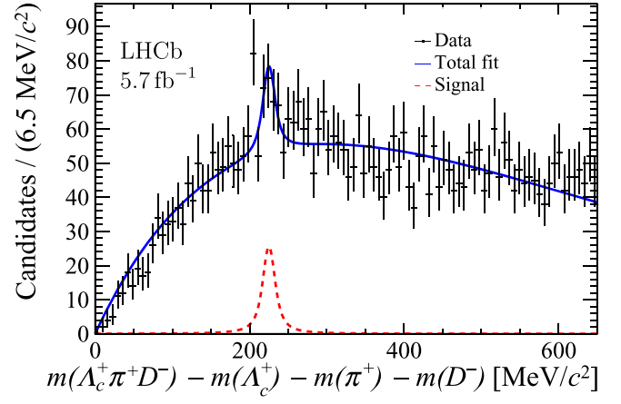
FIG. 6. Distribution of the Q value in the \Lambda_c^+ \pi^+ D^- channel, where the most significant signal is seen. The fit result is overlaid.
