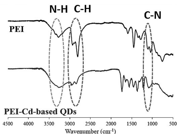
Figure 5: FT-IR spectra of PEI-capped QDs and PEI ( left ) and chemical structure of PEI ( right ).
