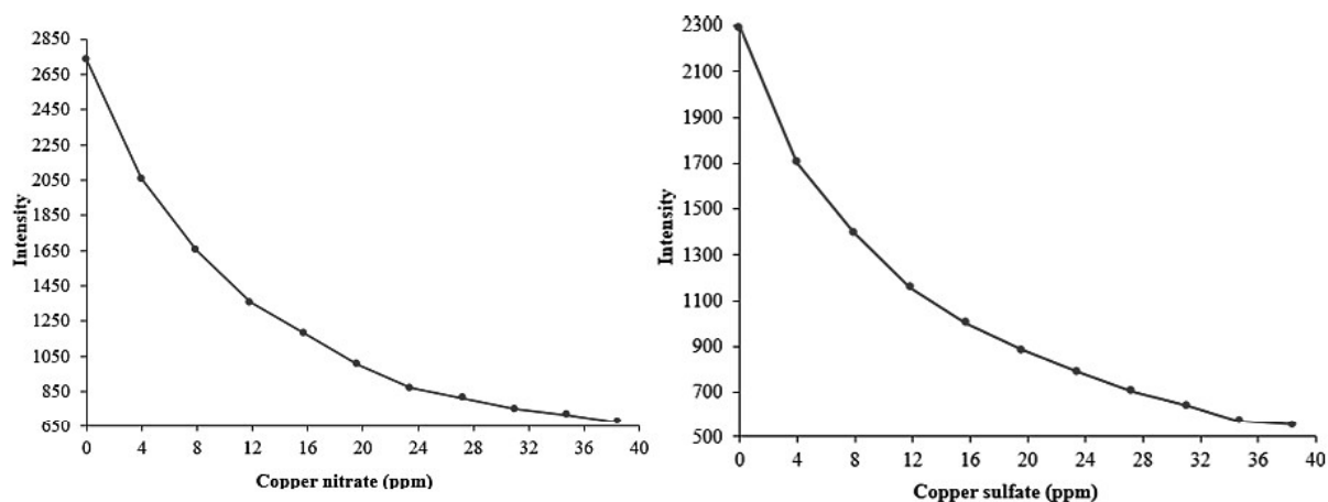
Figure 7: Sensing experiments with different copper solutions ( copper nitrate at the left and copper sulfate at the right ), in the presence of PEI-capped QDs.
