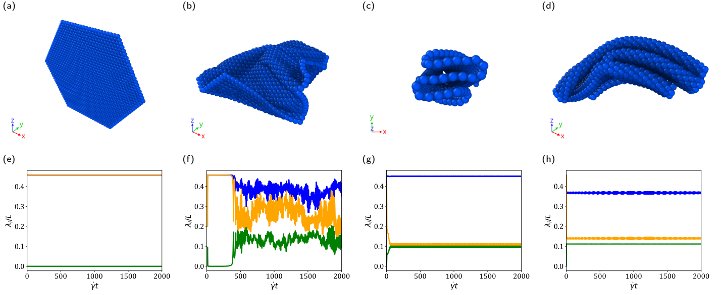
Fig. 1 (a-d) Example conformations for (a) flat, (b) tumbling, (c) 1D folded, and (d) 2D folded sheets. x is the flow direction and y is the shear direction. (e-h) Square root of the eigenvalues of the gyration tensor, \lambda_i , over time for the (e) flat, (f) tumbling, (g) 1D folded, and (h) 2D folded sheets. Green is the smallest, orange is the second largest, and blue is the largest characteristic length.
