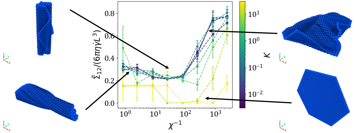
Fig. 6 Stresslet ("sheet viscosity") averaged over the last 200\dot{\gamma}\tau and all \phi . Error bars are 95% confidence intervals. Dotted lines drawn to guide the eye. On the borders are characteristic behaviors for different regions. x is the flow direction and y is the shear direction. Top left: high alignment folded. Bottom left: low alignment folded. Top right: tumbling. Bottom right: flat.
