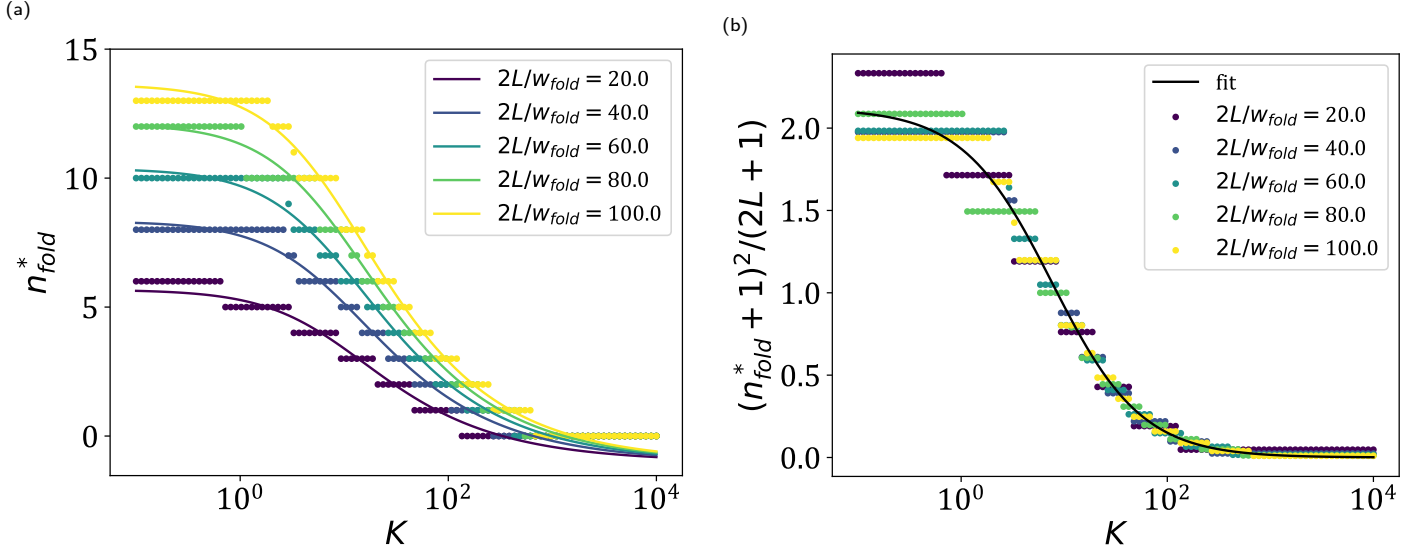
Fig. 8 (a) Optimal number of folds for varying K and L/w_{fold} . Points are data points and solid lines are Equation 24. Optimal values of \alpha and \beta were found to be \alpha = 0.0209 \pm 0.0004 and \beta = 0.539 \pm 0.003 using least-squares regression with R^2 = 0.989 . (b) Master curve using Equation 24 to collapse all plots of n_{fold}^* .
