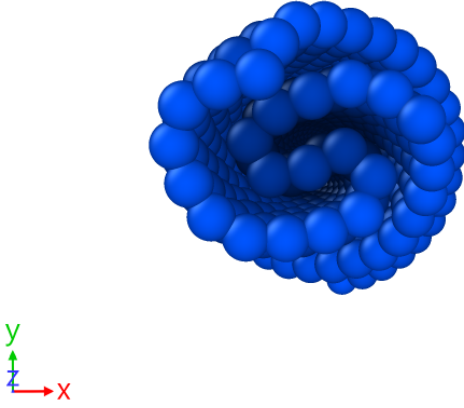
Fig. 5 Example of a 1D folded sheet that adopts a rolled-up conformation. x is the flow direction and y is the shear direction.
