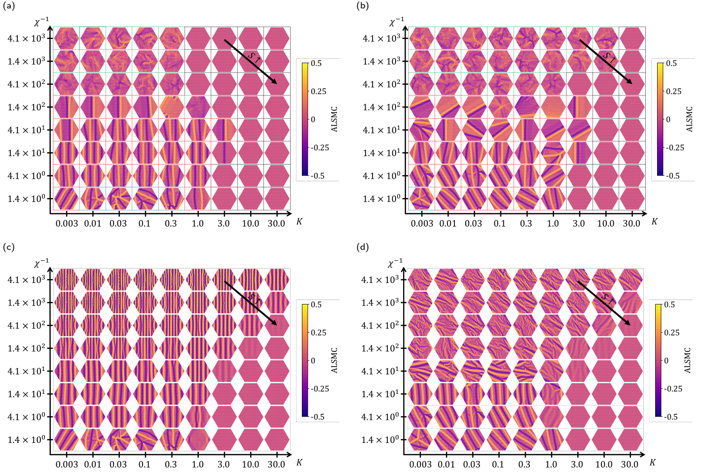
Fig. 4 Average signed local mean curvatures for sheets during the last 200\gamma t with (a) \phi = 0^\circ and (b) \phi = 45^\circ . Signed local mean curvatures for sheets at their initial flip with (c) \phi = 0^\circ and (d) \phi = 45^\circ . Diagonal lines running up and to the right correspond to sheets with constant S . Moving right or down corresponds to increasing S by about a factor of 3. The arrow in the top right corner of each plot indicates the direction of maximally increasing S . For reference, the sheet at K = 1.0 , \chi^{-1} = 1.4 has S \times 10^5 = 153 .
