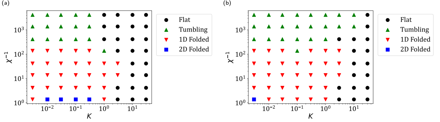
Fig. 2 Conformational phase map of sheets with initial conditions (a) \phi = 0^\circ and (b) \phi = 45^\circ .
