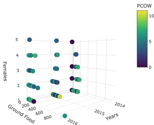
FIGURE 4 Per capita offspring weaned (PCOW) of females (for the two study sites combined) as a function of the interaction between biomass of edible vegetation (ground food, g/m 2 ) and the total number of females per social unit (Number of females), split by the random effect of year. On the color scale, high PCOW is indicated by green-yellow and low PCOW is indicated by dark blue-purple tones. The outlier point (>800 food) is a single female in 2016. Guidance for interpreting 3-D figures and supplemental 2-D figures are provided in Appendix S1.
