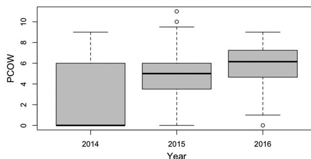
FIGURE 2 Box plot showing distribution of per capita offspring weaned (PCOW) by year for the two study sites combined. Visually, PCOW is lowest in 2014 due to the lack of offspring production at Parque Nacional Bosque Fray Jorge (PNBFI). There was a statistically significant random effect of year in models 2 and 3, indicating that fixed effects should be evaluated within each year. The total number of social units examined across both study sites were 29 in 2014, 31 in 2015, and 36 in 2016.
