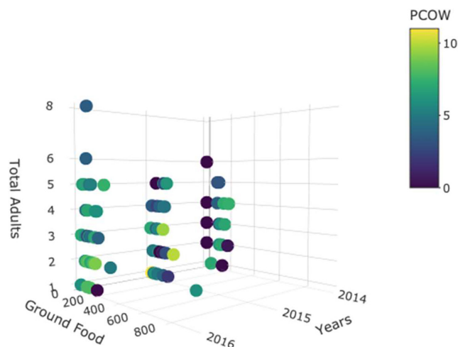
FIGURE 3 Per capita offspring weaned (PCOW) by females (for the two study sites combined) as a function of the interaction between biomass of edible vegetation (ground food, g/m 2 ) and the total number of adults per social unit, split by the random effect of year. On the color scale, high PCOW is indicated by green-yellow and low PCOW is indicated by dark blue-purple tones. The outlier point (>800 food) is a unit of two adults in 2016. Guidance for interpreting 3-D figures and supplemental 2-D figures are provided in Appendix S1.
