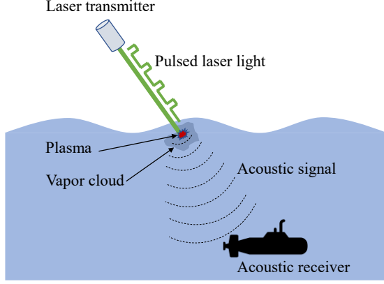
Fig. 1. Photoacoustic mechanism for air-to-underwater communication
