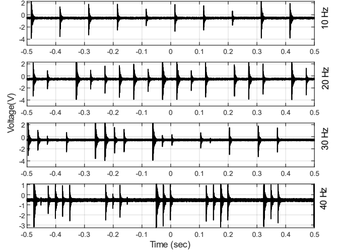
Fig. 2. Effect of vapor cloud on laser pulse repetition rate
