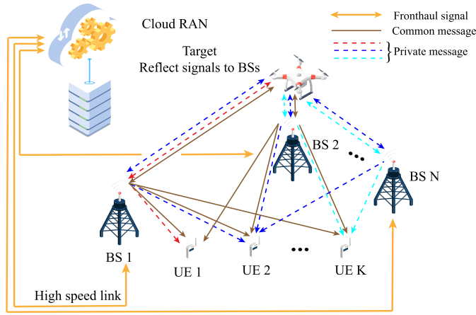
Fig. 27. The CoISAC system with RSMA transmission scheme and direct localization. K users while estimating a target's location [308].
