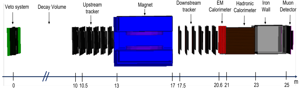
Figure 1: FASER-2 detector Geant4 simulation. From left to right, it comprises a veto system, a large cuboid decay volume, followed by a spectrometer composed of a large 1T magnet [10] with 6 tracking stations based on LHCb’s SciFi detector [11] each upstream and downstream, electromagnetic and hadronic dual-readout calorimeters [12], an iron wall, and a muon detector for particle identification and precise muon reconstruction.
