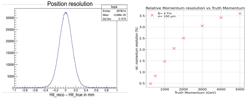
Figure 2: Simulation of 50 000 muons using ACTS toolkit to evaluate track reconstruction performance with the nominal FASER-2 geometry described in 1 . Left: Position resolution of each hits in the simulated trackers after the effect of the detector resolution modeled by a gaussian of \sigma = 100 \mu\text{m} . Right: Plot of the momentum resolution \sigma(\frac{p_{\text{reco}} - p_{\text{truth}}}{p_{\text{truth}}}) of muons from 200 MeV to 5 TeV simulated using particle gun
