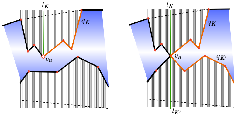
Figure 16. Two examples of Y_{n+1} and the corresponding \lambda^+ arcs and \Delta_i arcs. In the first case, the point v_n is a puncture so only one leaf l_K and path q_K is needed. In the second case, v_n lies on the boundary of two components of \text{int}_\tau(Y_0) \setminus Y_{n+1} .
