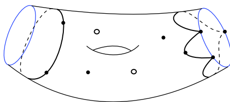
Figure 3. The image of a q -compatible subsurface Y in \bar{X}_Y under \hat{i}_q . Open circles are points of \tilde{\mathcal{P}}_Y (corresponding to the image of \partial_0 Y ), and dots are singularities not contained in \tilde{\mathcal{P}}_Y . The ideal boundary of X_Y is in blue.
