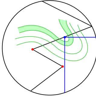
Figure 9. The component C_Y (green) and its intersection with l^\pm (blue). The intersection of the black zig-zag arc with \tilde{X} give components of \partial C_Y^\tau .
