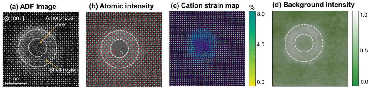
Figure 4 (a) Atomic-resolution ADF image of a single core-shell ion track. (b) Atomic intensity map from (a) to identify the respective Sr (red) and Ti (cyan) positions. (c) Cation strain map obtained from coordinates deduced from (b). (d) Corresponding background intensity map. The dotted circles depict the original ion track in the frame 0 corresponding to background intensity.
