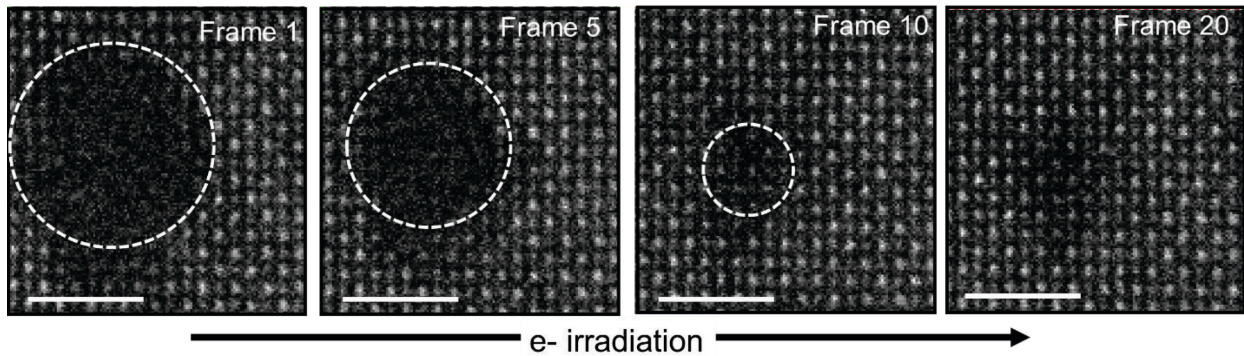
Figure 7 HAADF images showing the radially inwards recrystallization of amorphous ion-tracks in \text{SrTiO}_3 with subsequent e- beam irradiation. The circles in each image represent the decreasing amorphous regions of the ion-track. The scalebar shown in each image is of 2 nm.
