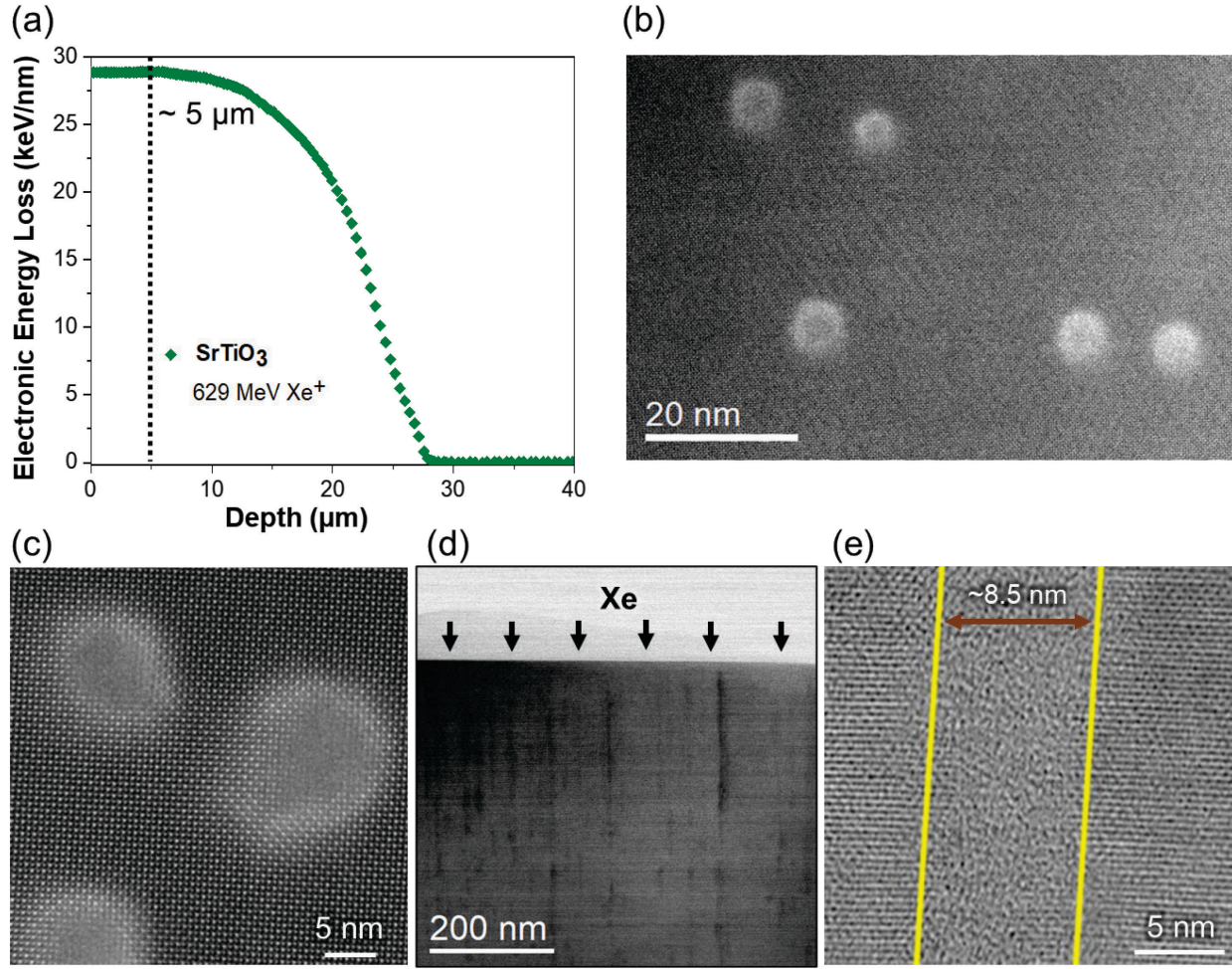
Figure 3 (a) Electronic energy loss as a function of penetration depth in SrTiO 3 after 629 MeV Xe ion irradiation. (b) Plan-view ADF image revealing core-shell ion track formation (acquired at the depth of ~5 \mu\text{m} ). (c) Atomic resolution ADF image of three ion-tracks revealing the formation of a core-shell track structure. (d) Cross-sectional annular bright-field (ABF) image of parallel oriented ion tracks embedded in SrTiO 3 . (e) Cross-sectional ABF image illustrating the amorphous structure of an individual cylindrical track.
