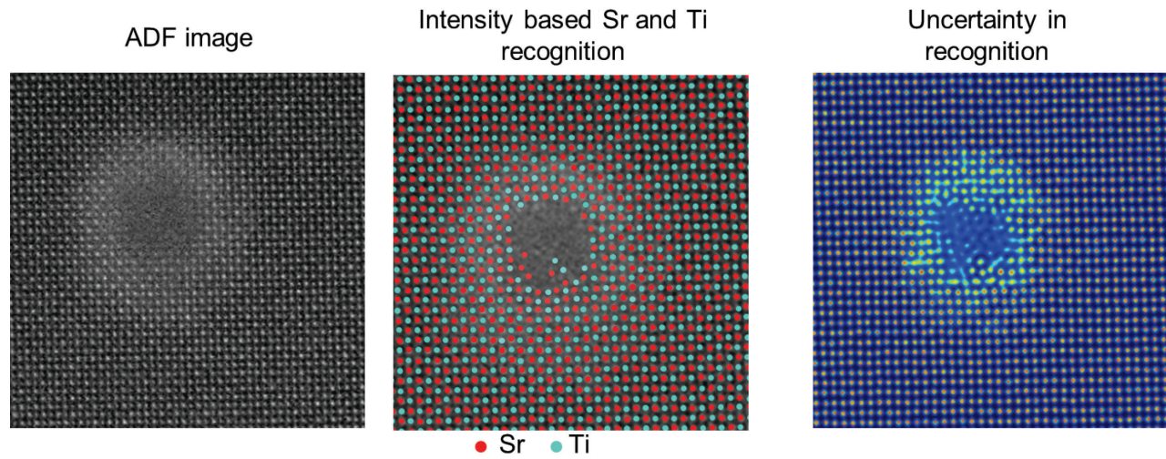
Figure 2 ADF image of the sample region containing an individual amorphous ion-track in \text{SrTiO}_3 . Image analysis yields identification of Sr (red) and Ti (cyan) atoms (middle image) and recognition uncertainty in the atomic features.
