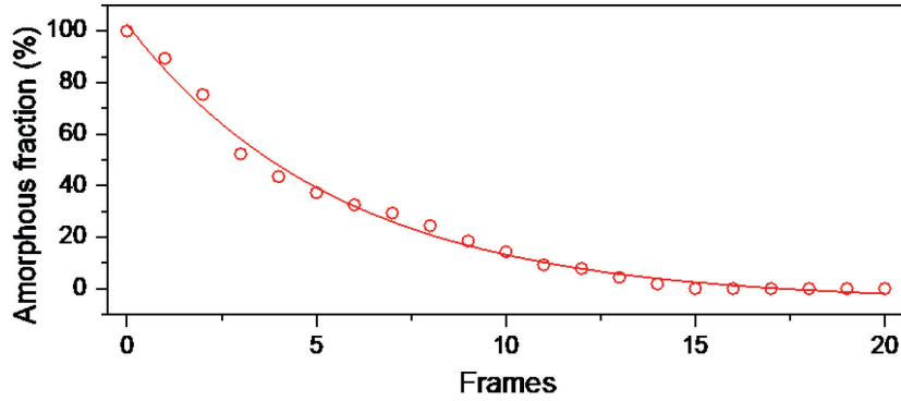
Figure 8 Variation of the amorphous phase as a function of acquired frames during the process of electron beam recrystallization. The positions of Sr and Ti atomic columns are determined for each frame (i.e frame 0- frame 20) to estimate the variation of amorphous phase with acquired frames revealing faster recrystallisation in early stages which slowed down in the later frames.
