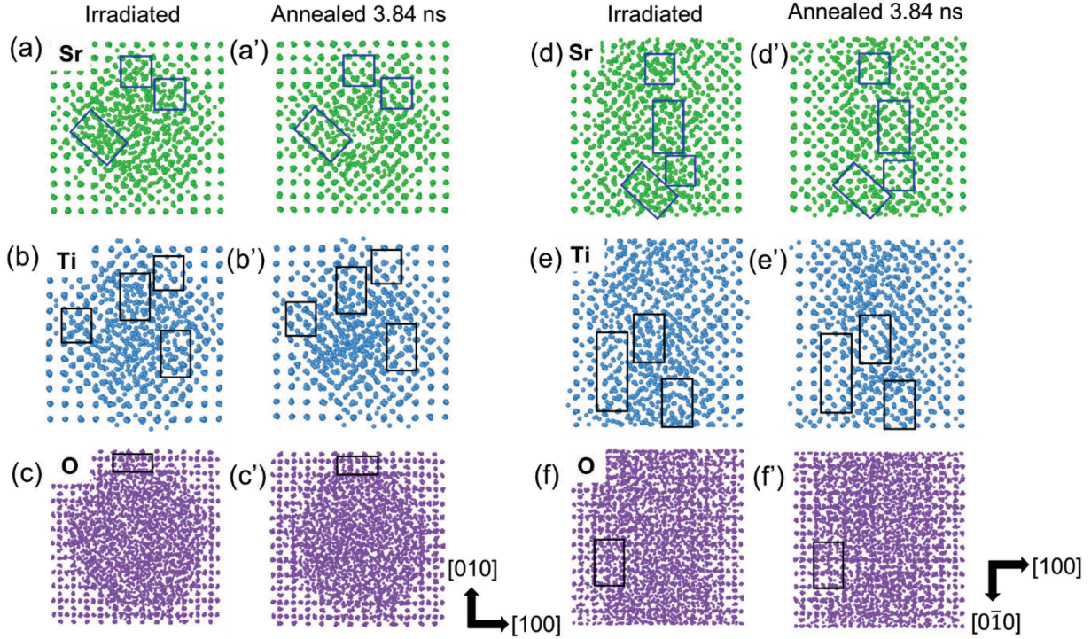
Figure 9 MD-simulated ion track formation after 629 MeV Xe irradiation and its annealed structure after annealing at 5000 K. The MD-simulated results are captured for Sr, Ti, and, O atoms, respectively. The arrangement of Sr, Ti, and O atoms after Xe irradiation and e-beam irradiation annealed structure is captured: (a-c) plan view of MD-simulated structure, and (d-f) cross-sectional view of MD-simulated structure. The corresponding annealed structures are shown in (a'-f').
