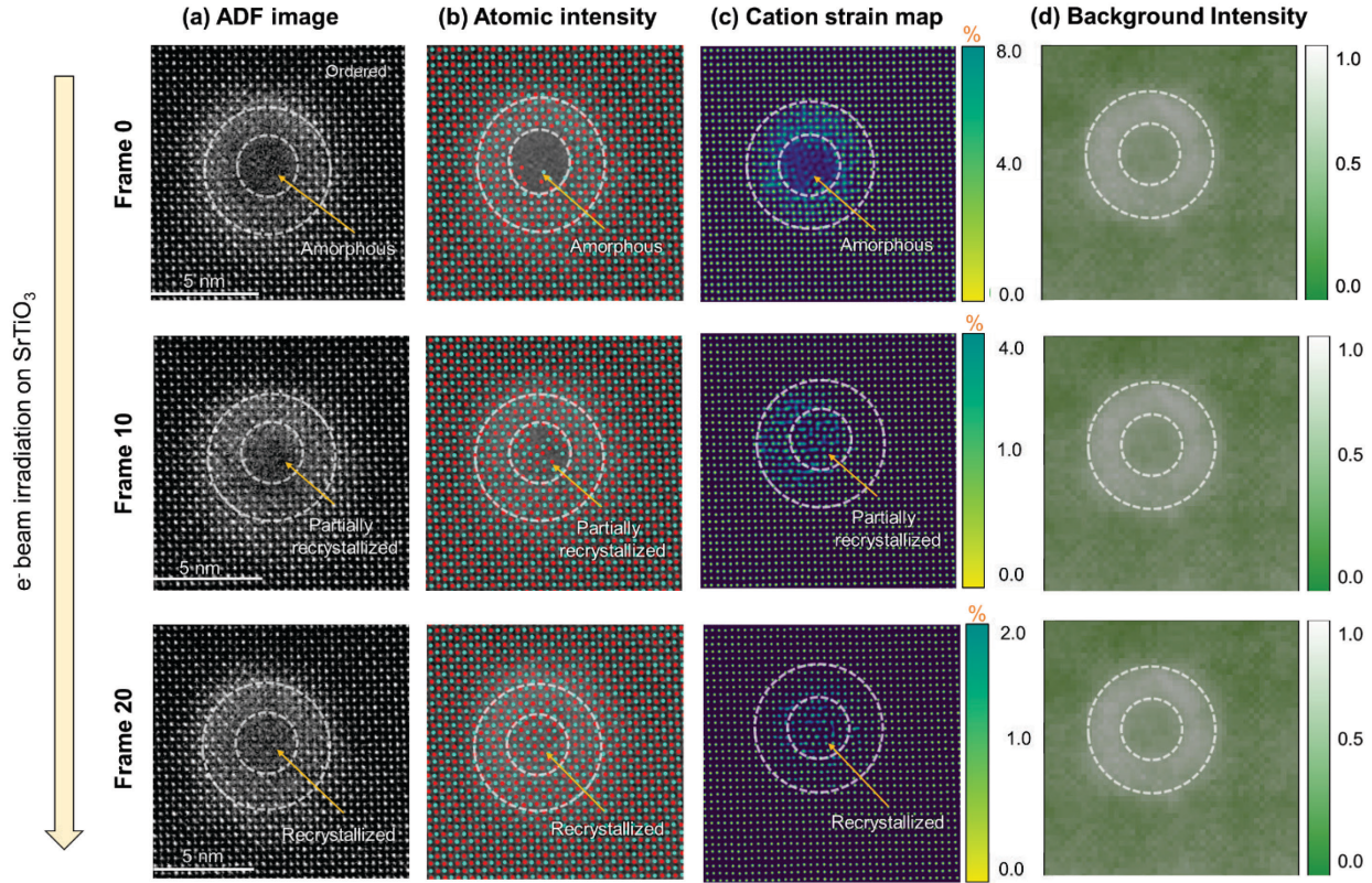
Figure 6 (a) ADF images showing amorphous ion-track recrystallization progression in Frame (image) 0, 10 and 20 out of a total of 20 frames acquired of the ion-track. The recrystallization process was completed within 20 frames. (b) Atomic intensity map from the corresponding ADF image to identify the Sr and Ti positions, indicated by red and cyan colors, respectively, (c) Cation strain map obtained from coordinates determined in Figures shown in (b), (d) Background intensity maps corresponding to ADF images acquired with e^- beam irradiation. The dotted circles in all the images represent the amorphous and disordered regions of the original ion track as observed in frame 0. These circles can be seen as guidelines to observe the changes in recrystallized regions (both in cationic strain and background intensity representing anion strain) after e^- beam irradiation with respect to the Frame 0.
