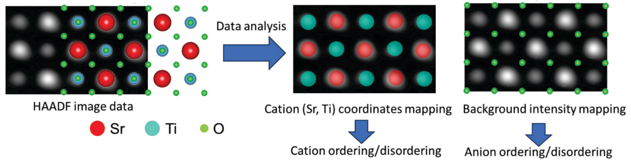
Figure 1 (a) Atomic resolution ADF image with overlaying SrTiO 3 atomic model in [001] surface normal direction consisting of Sr (red), Ti (cyan), O (green) circles, (b) atomic columns of cations (Sr, Ti) extracted from intensity analysis of (a) yielding information on cation disordering, (c) map of extracted background intensity representing anionic (O) disordering.
