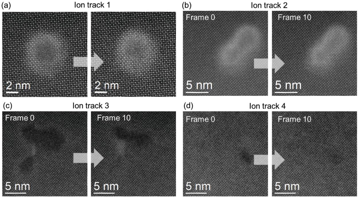
Figure 5 Examples of in situ electron-beam recrystallization of amorphous ion-tracks after scanning and acquiring 10 frames of images. The regions represent ion-tracks formed by (a) a single ion, (b) two ions, (c) multiple ions in the vicinity and (d) a single ion stochastically creating a smaller amorphous region.
