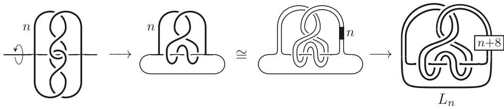
FIGURE 4 A link L_n whose branched double cover is S^3_1(5_2) . We quotient 5_2 by a rotation \tau around the indicated axis of symmetry, simplify the resulting diagram by an isotopy, and then replace the arc 5_2/\tau by a rational tangle. The box labeled “ n + 8 ” corresponds to n + 8 signed half-twists.
