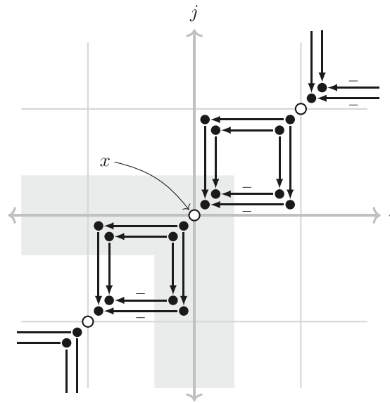
FIGURE 3 The complex (CFK^{\infty}(K), \partial^{\infty}) , with \hat{A}_0 shaded and possible diagonal arrows omitted. The black dots represent generators of C\{i, j\} in grading m_0 + i + j , while the white dots represent generators U^{-i}x in grading i + j . The minus signs on some arrows indicate a coefficient of -1 in \partial^{\infty} .
