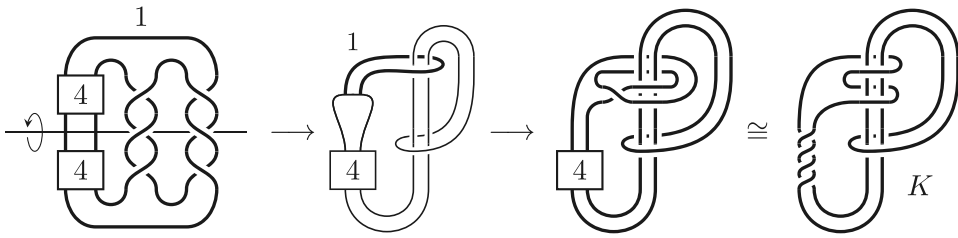
FIGURE 5 Identifying S_1^3(P(-3, 3, 8)) as a branched double cover \Sigma_2(K) . We quotient P(-3, 3, 8) by a rotation \tau around an axis of symmetry and simplify by an isotopy, following [4, Figure 7]. We then replace a neighborhood of the arc P(-3, 3, 8)/\tau with a rational tangle, and isotope further to get the desired knot K .
