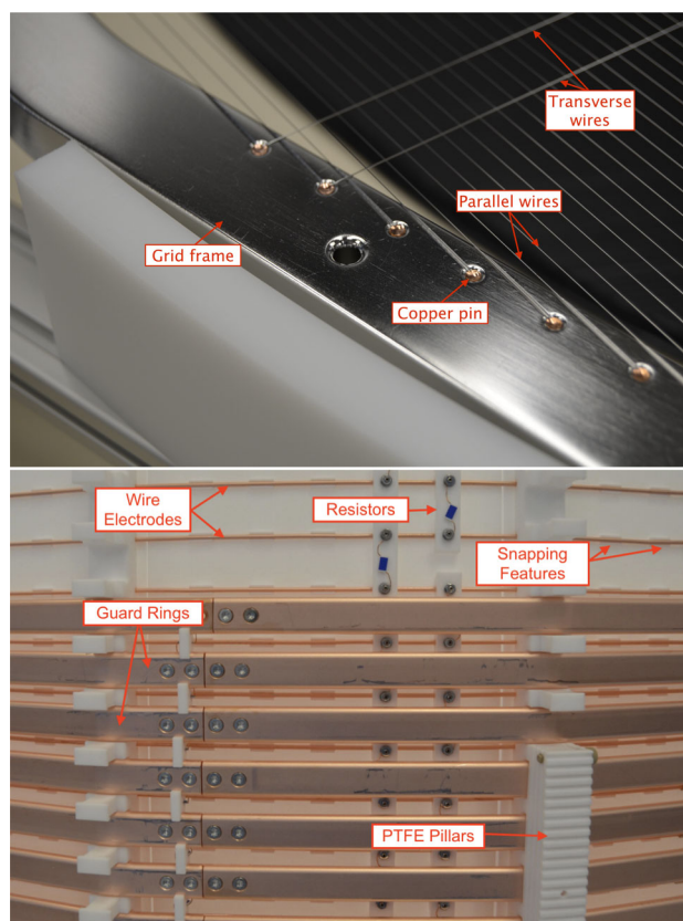
Fig. 7 (top) The electrode wires are individually fixed by copper pins to the electrode frames (here: anode). Two transverse wires, installed to reduce sagging, are shown as well. (bottom) Detailed outside view of the TPC field-shaping elements during installation: the massive guard rings (15 mm height) and the thinner wire field electrodes (2 mm diameter) are installed at half pitch at different distances from the 3 mm thick PTFE reflectors. The guard electrodes consist of two pieces fixed together by two M3 SS bolts at each junction. The other two bolts are used to fix the guard-ring resistor chain (installed within the guard rings). Also visible are the 5 G \Omega resistors on PTFE supports connecting the wire field electrodes
