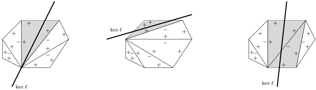
Fig. 2. Half-open triangulations of a polygon in the cases where \ker \ell intersects the boundary of the polygon in a vertex and the interior of a side (left) or two sides (middle/right). Removed/open faces are denoted by “-”, closed/non-removed faces with “+”. The convex hull of the corresponding vertex/sides is depicted in gray. All half-open triangles violate conditions (i) and (ii) of Lemma 3.2.
