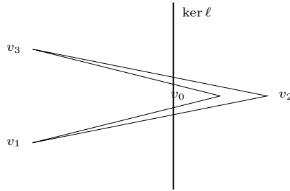
Fig. 3. Example of a non-convex lattice quadrilateral that has an h^* -polynomial with negative coefficients with respect to a weight w(x) = x_1^2 .
