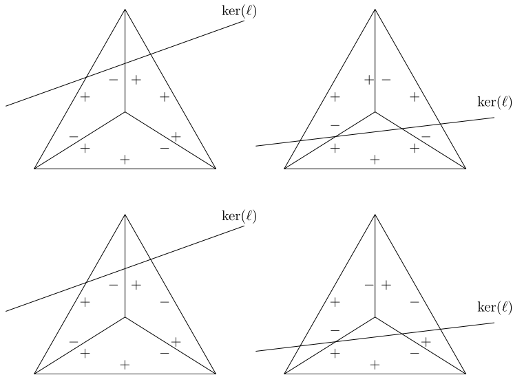
Fig. 1. Subdivision of triangle using an internal integer point. Each edge is marked with + or – to indicate which simplex includes it; the simplex containing + contains the edge and the simplex containing – excludes it.
