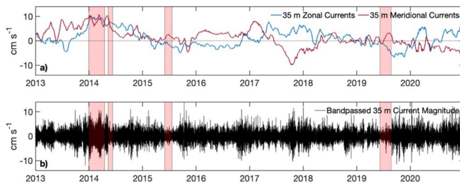
Figure 7. (a) Total zonal and meridional 35 m currents [ \text{cm s}^{-1} ] and (b) near-inertial 35 m current magnitudes [ \text{cm s}^{-1} ] observed from the NOAA surface mooring at OSP. The zonal and meridional current data are shown as a 31-day running average. The red shading represents observed MHW periods.
