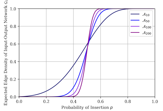
Fig. 1. Polarization behavior of expected edge density for certain codebooks over deletion and insertion channels. Exact formulas for edge densities are given in Theorems 9 and 20. Figure 1(d) is obtained from Theorem 20 in Section V.
