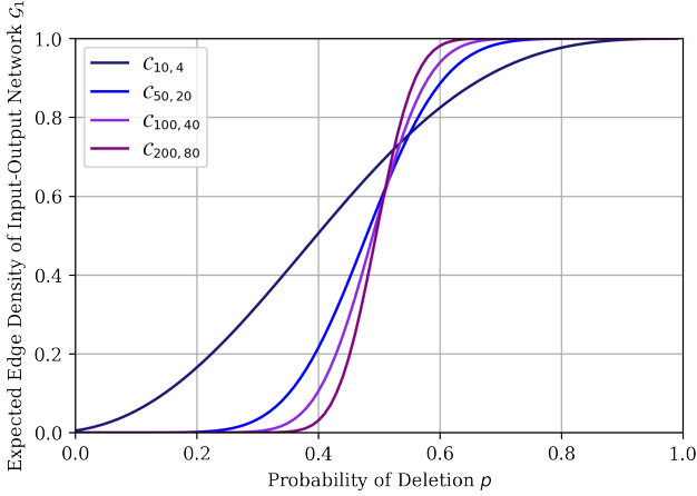
Fig. 1. Polarization behavior of expected edge density for certain codebooks over deletion and insertion channels. Exact formulas for edge densities are given in Theorems 9 and 20. Figure 1(d) is obtained from Theorem 20 in Section V.
