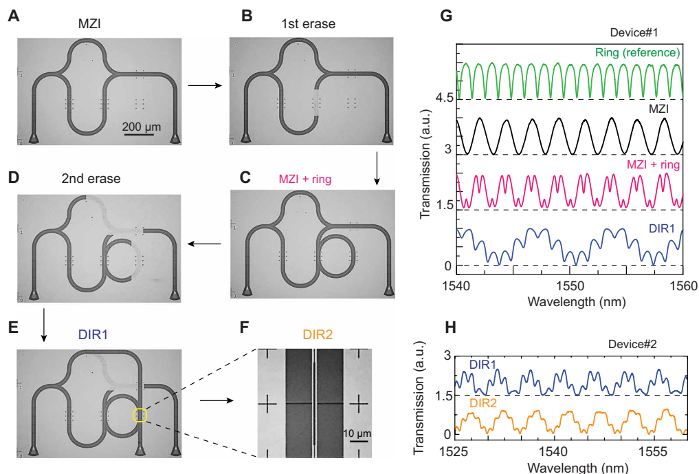
Fig. 4. Shaping the spectral response of an optical filter in steps. (A) An MZI written by DLW on a Sb 2 Se 3 thin film. (B) Erase part of the bottom arm of the MZI. (C) Add a ring resonator to the erased region of the MZI. (D) Erase part of the ring resonator and the MZI. (E) Reconnect the device as the DIR filter. (F) Tuning the coupling by increasing the gap between the ring resonator and the top arm of the Y-splitter. (G) The transmission spectra of the optical filter after each reconfiguration step. Spectra have been vertically translated for clarity. (H) The transmission spectra of the DIR filter before (blue curve) and after (orange curve) tuning the ring resonator coupling.
