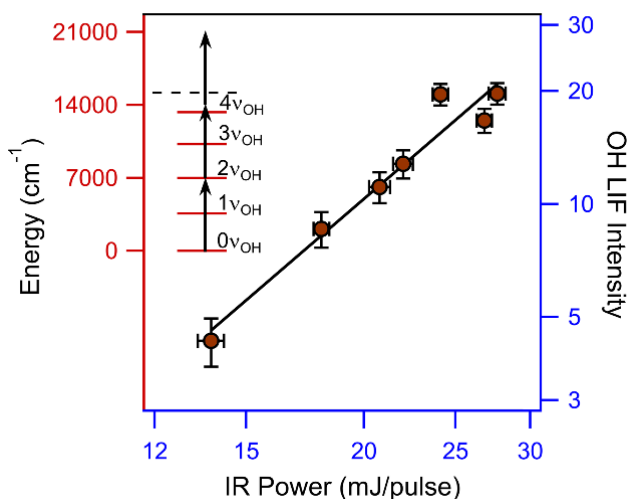
Figure 3. (Left) Energy diagram showing the multiphoton dissociation of CHHP. IR excitation of the 2\nu_{\text{OH}} transition (black arrow) followed by absorption of additional photon(s) provides sufficient energy to exceed the O-O bond dissociation limit of CHHP (dashed line), resulting in cyclohexoxy and OH radicals. The OH radicals are detected by LIF on the A^2\Sigma^+ - X^2\Pi_{3/2}(1,0) Q_1(3.5) transition at 282 nm. (Right) IR-induced OH LIF signal intensity at 7012.5\text{ cm}^{-1} as a function of IR power (mJ/pulse). Both axes are plotted on a \log_{10} scale, yielding a slope of 2.3 \pm 0.3 . The nonlinear IR power dependence indicates multiphoton excitation of CHHP.
