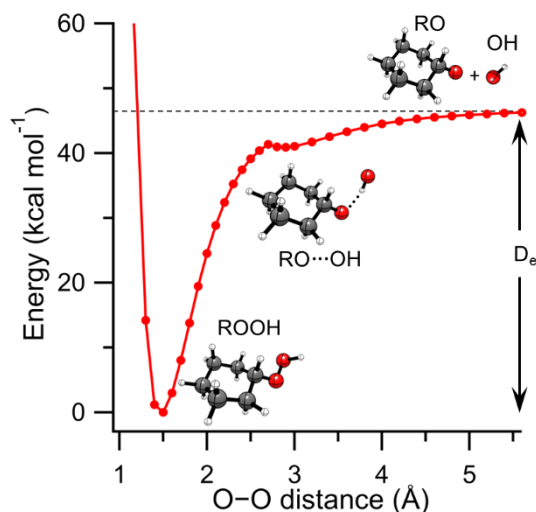
Figure 4. Energy diagram for the equatorial conformer of CHHP (ROOH) along the O–O stretch coordinate ( R_{OO} ) to form cyclohexoxy (RO) + OH products. The potential is calculated at the CASPT2/aug-cc-pVTZ level of theory. A bond dissociation energy ( D_e ) of 46 kcal mol −1 is obtained for the equatorial conformer of CHHP.
