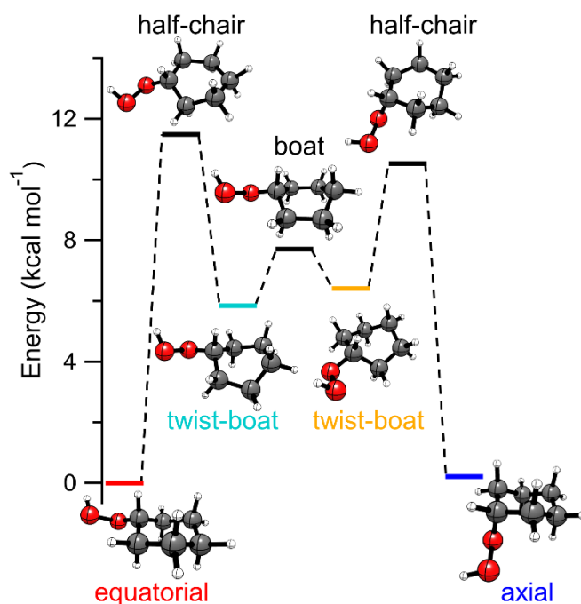
Figure 1. Energy profile connecting the equatorial and axial conformers of CHHP calculated at the CCSD(T)-F12/cc-pVTZ-F12//B2PLYPD3/cc-pVTZ level of theory.
