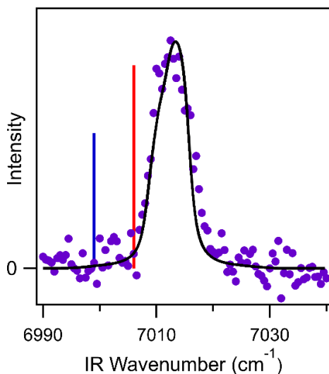
Figure 2. Theoretically predicted 2\nu_{\text{OH}} transitions for the equatorial (red) and axial (blue) conformers of CHHP at 7006 and 6999\text{ cm}^{-1} , respectively, shown with relative intensities of 60:40 for a room temperature Boltzmann distribution. Experimental IR action spectrum (purple points) is overlaid with a simulated rotational band contour (black) for a scenario of closely spaced 2\nu_{\text{OH}} transitions (ca. 3\text{ cm}^{-1} apart) for equatorial and axial conformers. A nearly indistinguishable simulation results from an alternate limiting case with IR power broadening of the 2\nu_{\text{OH}} transition for the equatorial conformer that increases the homogeneous linewidth to 6.0\text{ cm}^{-1} (see Figure S8). The spectral shift of the observed feature (ca. 10 \pm 2\text{ cm}^{-1} ) is within the accuracy of the theoretical predictions ( 10\text{-}20\text{ cm}^{-1} ).
