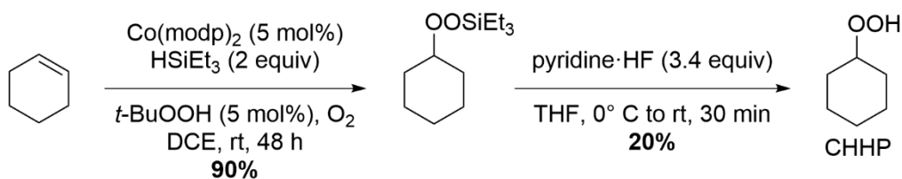
Scheme 1. Synthetic route to generate cyclohexyl hydroperoxide (CHHP).
