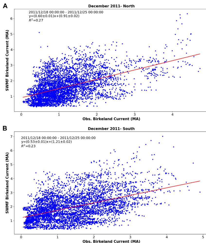
FIGURE 5 Observations and SWMF Birkeland current for December 2011. (A) Northern Hemisphere (B) Southern Hemisphere.
