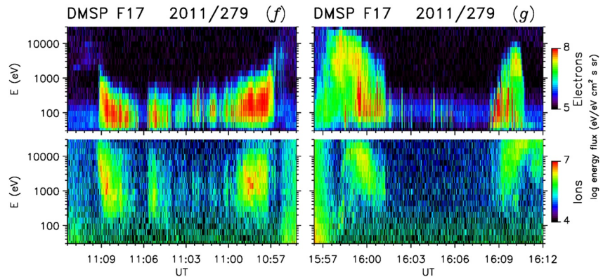
Figure 3. Spectrograms of precipitating electrons and ions measured by the SSJ/4 instrument from two passes of DMSP-F17, corresponding to panels (f) and (g) of Figure 2. The time axis of the left-hand spectrogram is reversed so dusk is to the left and dawn to the right in both cases.
