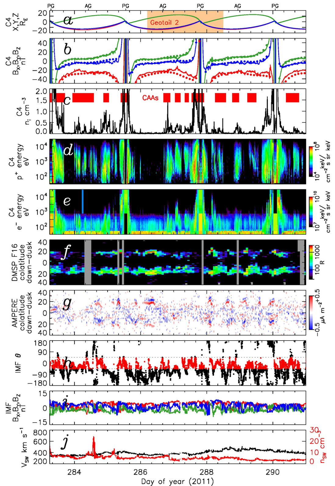
Figure 5. Observations from 10 to 17 October, presented in the same format as Figure 4.
