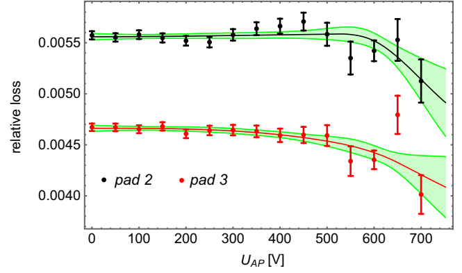
FIG. 1. Simulated fraction of undetected protons (both for pad 2 and pad 3 of the SDD) of the integral proton spectrum whose corresponding pulse heights fall below the threshold of the data acquisition system. The U_{AP} dependence of the simulated losses can be described by a cubic spline function (solid line) and is shown together with the 1\sigma error predicted by the global fit (green band).
