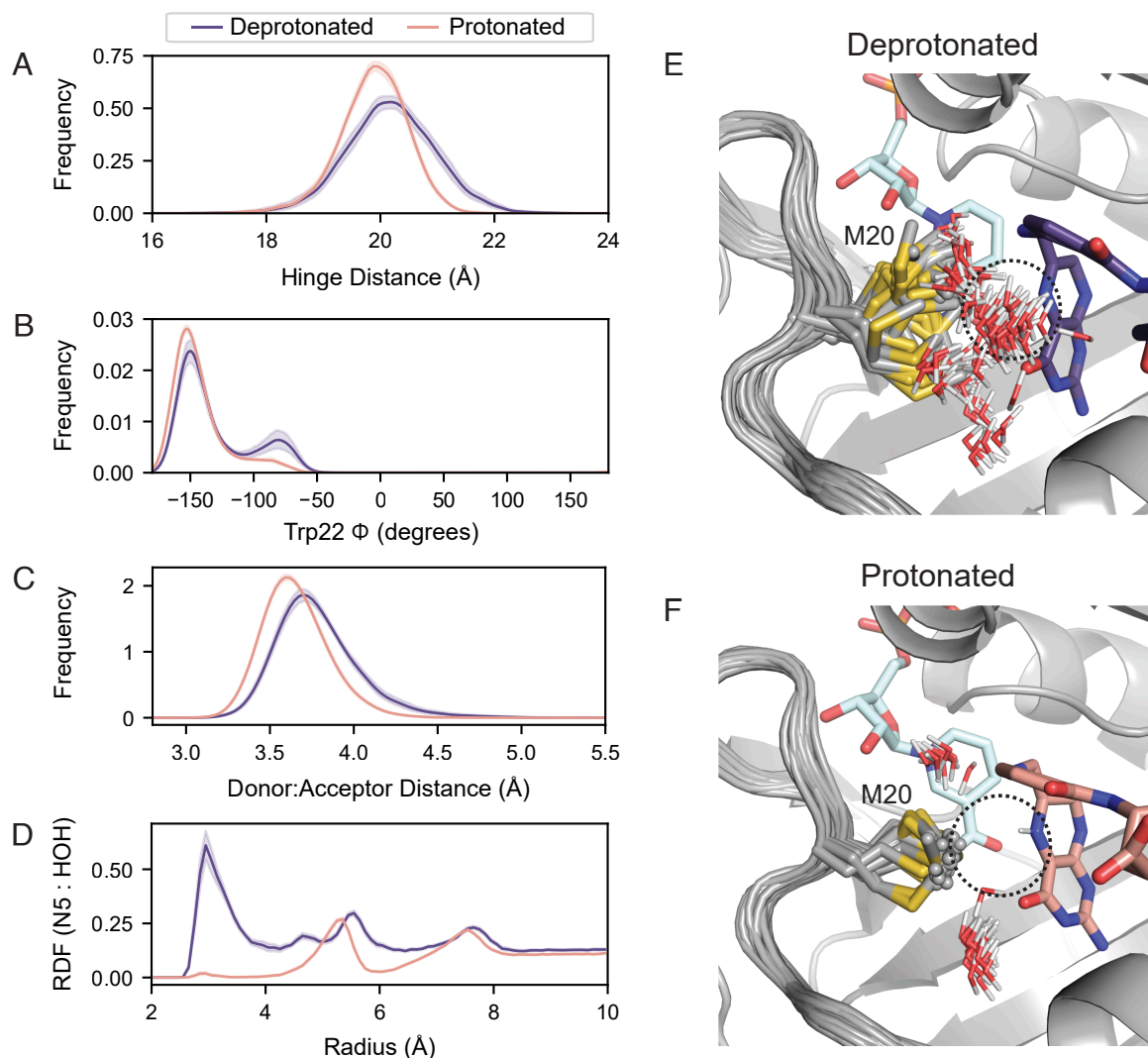
Fig. 6. Protonation of the substrate orders the Met20 sidechain in the Michaelis complex. Fifty independent MD simulations of the ecDHFR:NADPH:DHF complex, with and without protonation of the N5 nitrogen, were run for 100 ns each. Kernel density estimates of the (A) hinge distance, (B) Trp22- \phi , (C) donor–acceptor distance for hydride transfer change upon protonation of the substrate. These kernel density estimates were computed for each trajectory independently and the mean and 95% CI is shown for each condition. (D) The density of water around the N5 nitrogen of DHF as a function of distance from the N5 nitrogen RDF mean and 95% CI are shown. The first 50 frames (20 ns) from one trajectory are superimposed for the (E) deprotonated and (F) protonated substrate, depicting the Met20 sidechain and all waters within 4.5 Å of the N5 nitrogen of DHF. Only the initial frame is depicted for DHF and NADPH for visual clarity.
