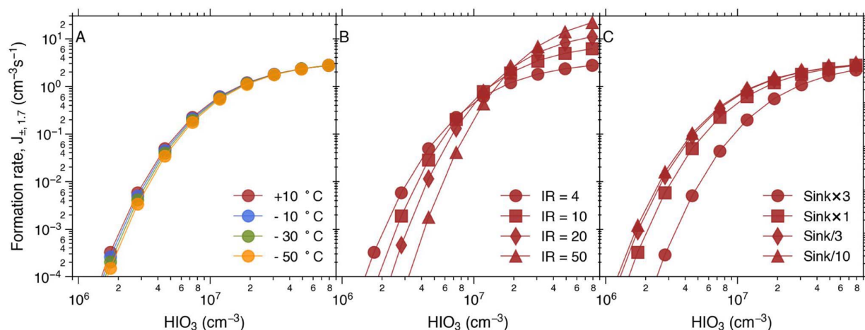
Fig. 3 The temperature (A), ionisation rate (B), and sink (C) dependence of J_{\pm} simulated by the PANDA520 model. If not stated otherwise the temperature is +10 °C, the ionisation rate is 4.1 \text{ ion pairs cm}^{-3} and the sink is 0.002 \text{ s}^{-1} . This shows that from these three parameters, the charged cluster formation rate is most sensitive to the ionisation rate. At \text{HIO}_3 concentrations below 1.5 \times 10^7 \text{ cm}^{-3} the impact of recombination loss is higher than the ion growth due to \text{HIO}_3 condensation and the formation rate decreases with increasing ionisation rate.
