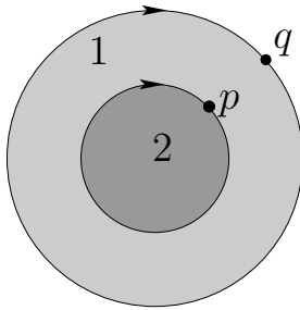
FIGURE 1.1. p is a two-sided point while q is a one-sided point.
