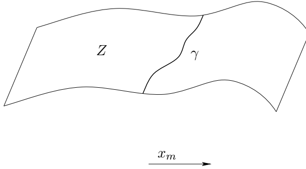
FIGURE 5.1. The current Z is the graph over \Omega^- of a function \psi' which does not depend on x_m : \psi' is chosen so that \partial Z = \llbracket \Gamma \rrbracket .
