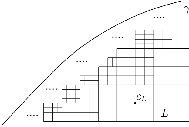
FIGURE 7.1. The Whitney decomposition \mathcal{W} in \Omega^- .
