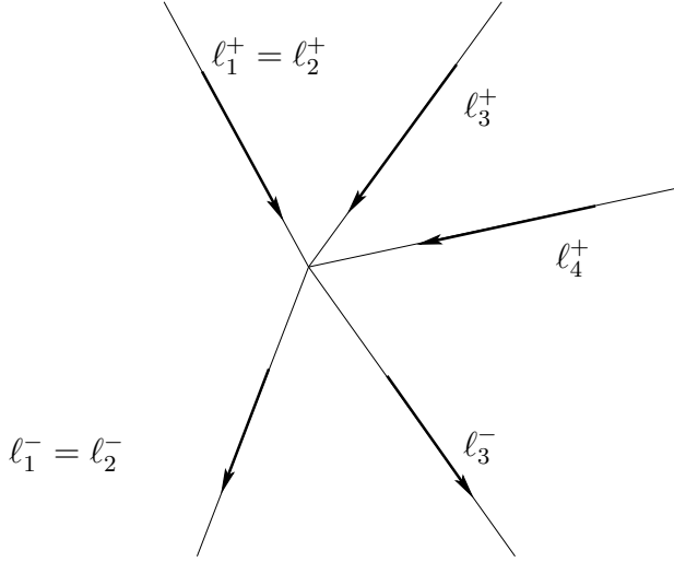
FIGURE 3.1. An example of current S and oriented lines \ell_j^\pm when Q = 4 : the arrows represent the oriented tangent to the lines. Note that pairs of lines \ell_j^+, \ell_k^+ and \ell_j^-, \ell_l^- might coincide: in the example we have \ell_1^+ = \ell_2^+ and \ell_1^- = \ell_2^- . However the support of any line \ell_j^+ can intersect the support of any line \ell_k^- only at the origin, otherwise (3.7) would be violated.
