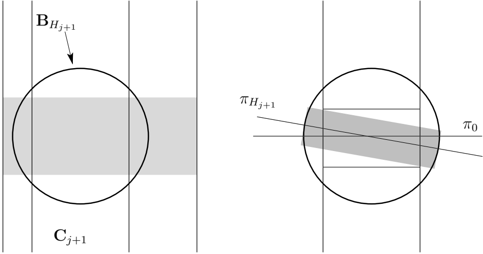
FIGURE 8.1. The inductive proof of (ii) j+1 consists of two steps: first the height bound in the cylinder \mathbf{C}_j is used to prove that \text{spt}(T) \cap \mathbf{C}_{j+1} \subset \mathbf{B}_{H_{j+1}} ; then the height bound in \mathbf{B}_{H_{j+1}} is used to prove the height bound in the cylinder \mathbf{C}_{j+1} .
