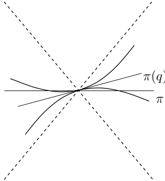
FIGURE 6.1. The region delimited by the thick curved lines is the right hand side of (6.9), whereas the cone delimited by the thick dashed straight lines is the right hand side of (6.8).
