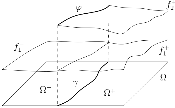
FIGURE 4.1. A \frac{3}{2} -valued function with interface (\gamma, \varphi) : the function f^+ is the 2-valued map \llbracket f_1^+ \rrbracket + \llbracket f_2^+ \rrbracket and f^- coincides with the (classical) single-valued f_1^- .
