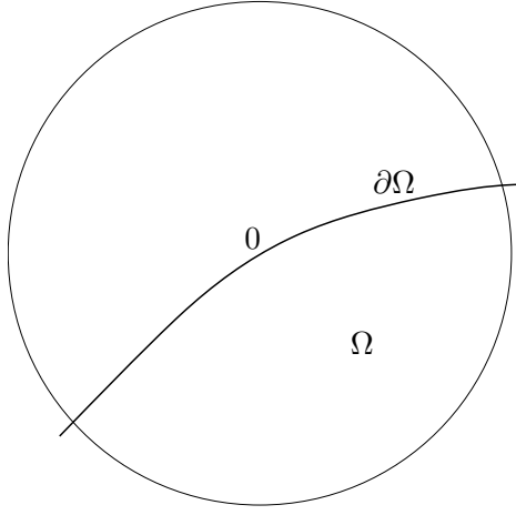
FIGURE 4.3. The domain \Omega . f in Theorem 4.15 collapses to Q \llbracket 0 \rrbracket on \partial\Omega .
