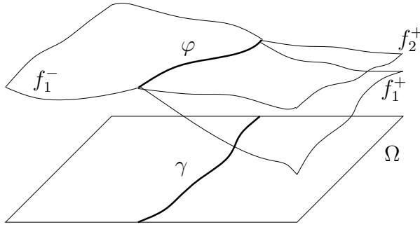
FIGURE 4.2. A \frac{3}{2} -valued function which collapses at the interface (\gamma, \varphi) .
