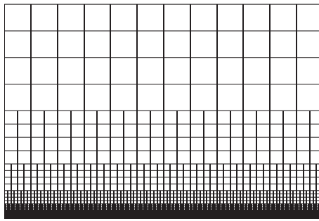
Fig. 1. The Whitney decomposition of [0, 2^{-N_0}] \times [-2, 2]^{m-1} . In the above example the parameter M equals 2.
