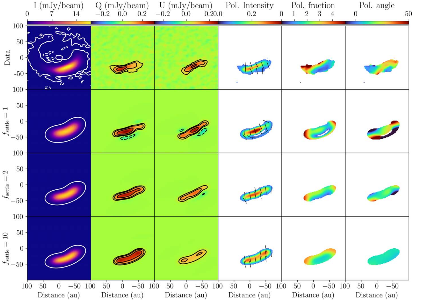
Figure 3. Detailed comparisons between the data and our models. From top to bottom, each row represents the data and models with f_{\text{settle}} = 1, 2 , and 10 , respectively. From left to right, each column represents Stokes I , Q , U , PI, polarization fraction, and polarization PA, respectively. For the Stokes I column, the contours represent \pm 3\sigma_I contours. For the Stokes Q and U columns, the contours are plotted at the levels of (-8, -4, 4, 8, 16) \times \sigma_{PI} . For the PI column, the line segments with uniform length represent the orientation of polarization. For the right three columns, only regions with PI > 4\sigma_{PI} are shown.
