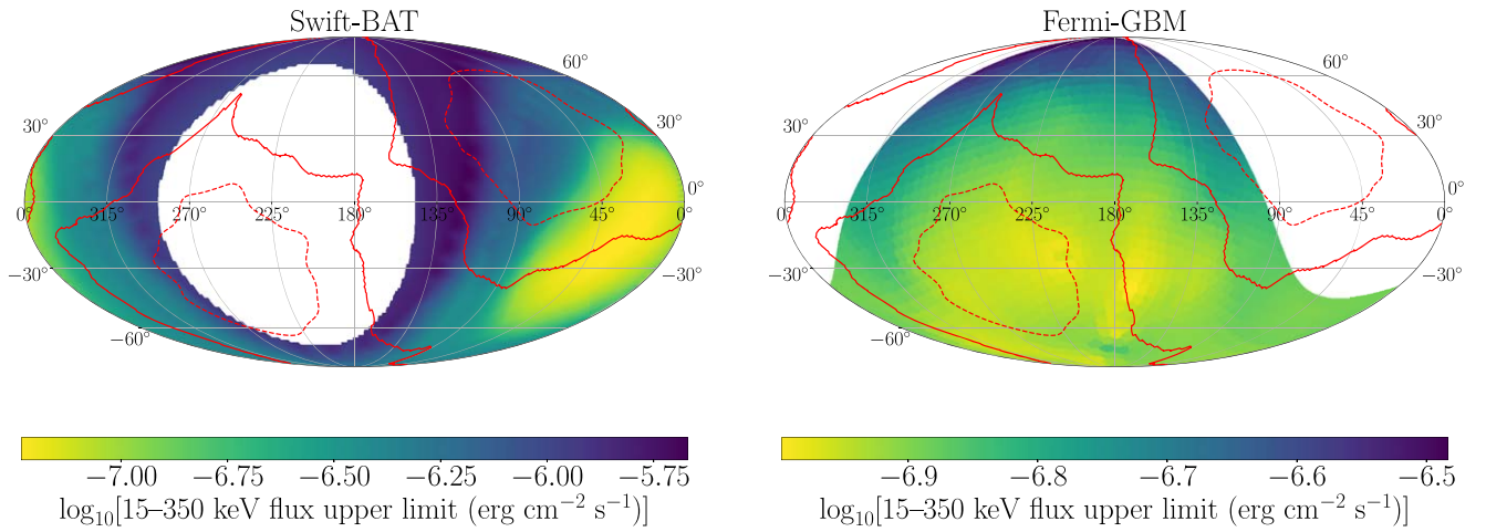
Figure 11. Upper-limit sky map in the 15–350 keV band for Swift-BAT (left) and Fermi-GBM (right). The upper limits are relative to a timescale of 1 s, computed at a 5\sigma confidence level. Solid and dashed lines are the GW contours at 90% and 50% credibility, respectively. The white region is the position of the Earth, for which no upper limits are available.
