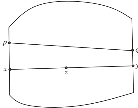
Figure 1. Figure for the proof of part (4) Case 4, when the convex hull of \bar{\ell}_1 \cup \bar{\ell}_2 is a two-dimensional 4-gon.
