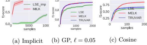
Figure 2: Performance of MELK and MILK versus Gaussian process baseline.
