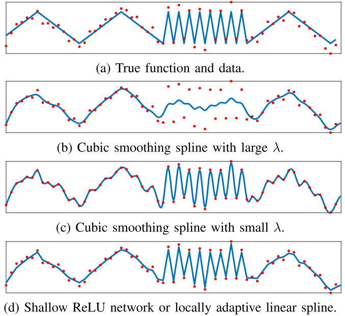
Fig. 1. In (a) we generate data from noisy samples of a function in BV^2[-1, 1] but not in H^2[-1, 1] . In (b) and (c) we fit the data using a cubic smoothing spline with both large and small \lambda . In (d) we fit the data using a locally adaptive linear spline which corresponds to training a shallow ReLU network (to a global minimizer) with weight decay (or path-norm regularization).
