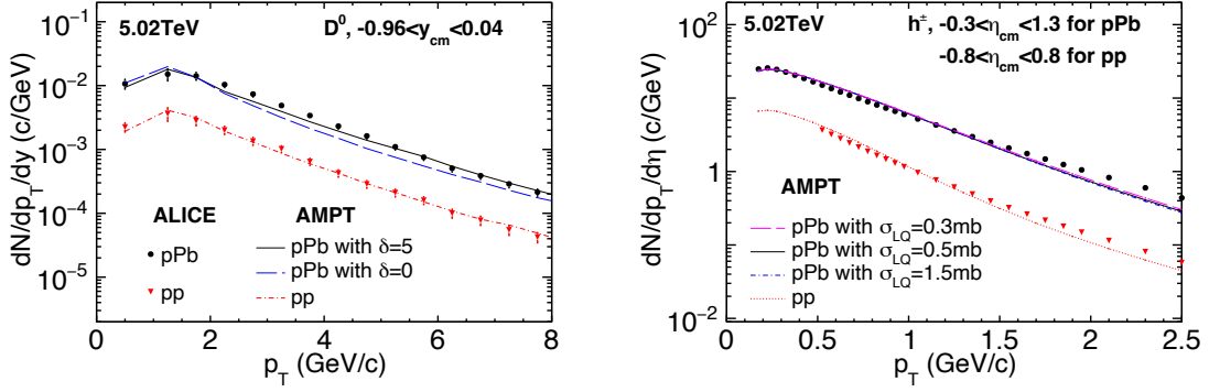
Figure 1: Left panel: AMPT model results on the transverse momentum spectra of D^0 mesons at mid-rapidity in p + p collisions and minimum bias p -Pb collisions (with \delta = 5 or 0 ) at 5.02 TeV in comparison with the experimental data. Right panel: transverse momentum spectra of charged hadrons around mid-rapidity in p + p collisions and p -Pb collisions at 5.02 TeV from the AMPT model in comparison with the experimental data. The AMPT spectra for p -Pb collisions are shown for three values of \sigma_{LQ} : 0.3, 0.5, and 1.5 mb.
