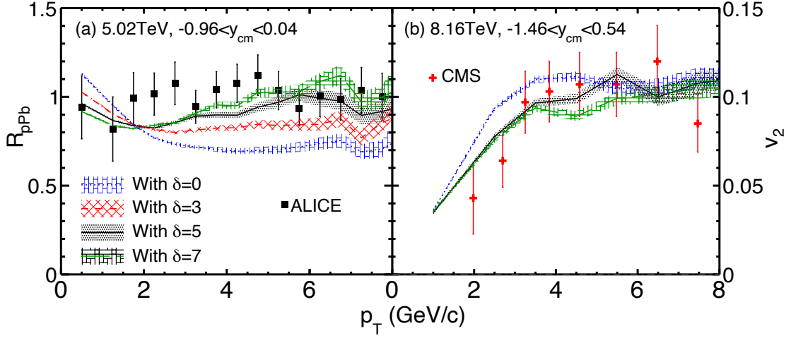
Figure 3: D^0 meson (a) R_{pPb} in minimum bias p -Pb collisions at 5.02 TeV and (b) v_2 in high multiplicity p -Pb collisions at 8.16 TeV from the AMPT model with different strengths of the Cronin effect ( \delta ) in comparison with the experimental data (symbols).
