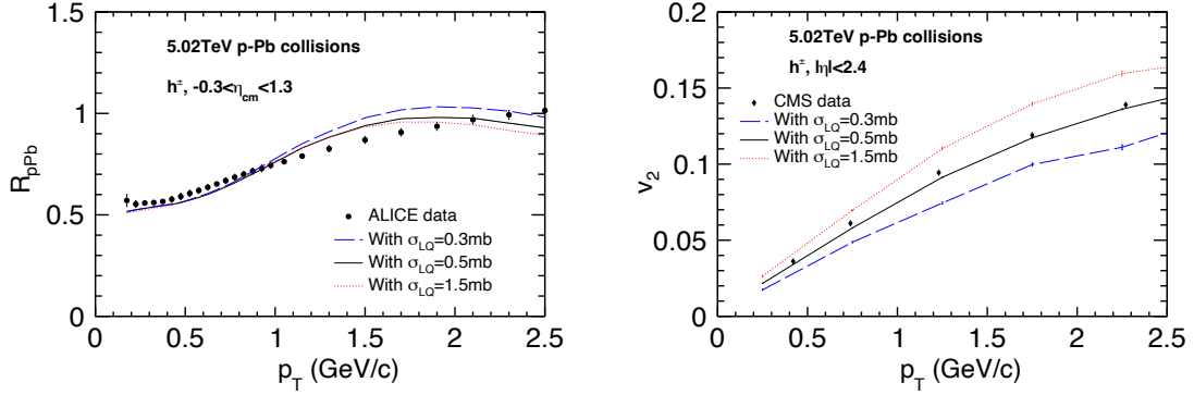
Figure 2: Charged hadron R_{pPb} (left panel) in minimum bias p -Pb collisions at 5.02 TeV and v_2 (right panel) in high multiplicity p -Pb collisions at 5.02 TeV from the AMPT model with \sigma_{LQ} = 0.3, 0.5 , and 1.5 mb in comparison with the experimental data.
