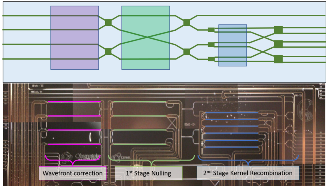
Figure 37. A schematic of a 4-input Kernel nullo device (top) achieved by the use of traditional waveguides, 2 \times 2 directional couplers, and 1 \times 2 splitters (green). TOPAs (colored) are used to control the internal path length matching of the interferometer arms inside the chip and correct for any error coming from either outside the chip (pink), inside the first stage nulling (green), and the beam-recombination that creates the kernel nulls. Microscope image (bottom) of the fabricated device, on a silicon nitride platform. Here the TOPAs are colored to their corresponding function.
