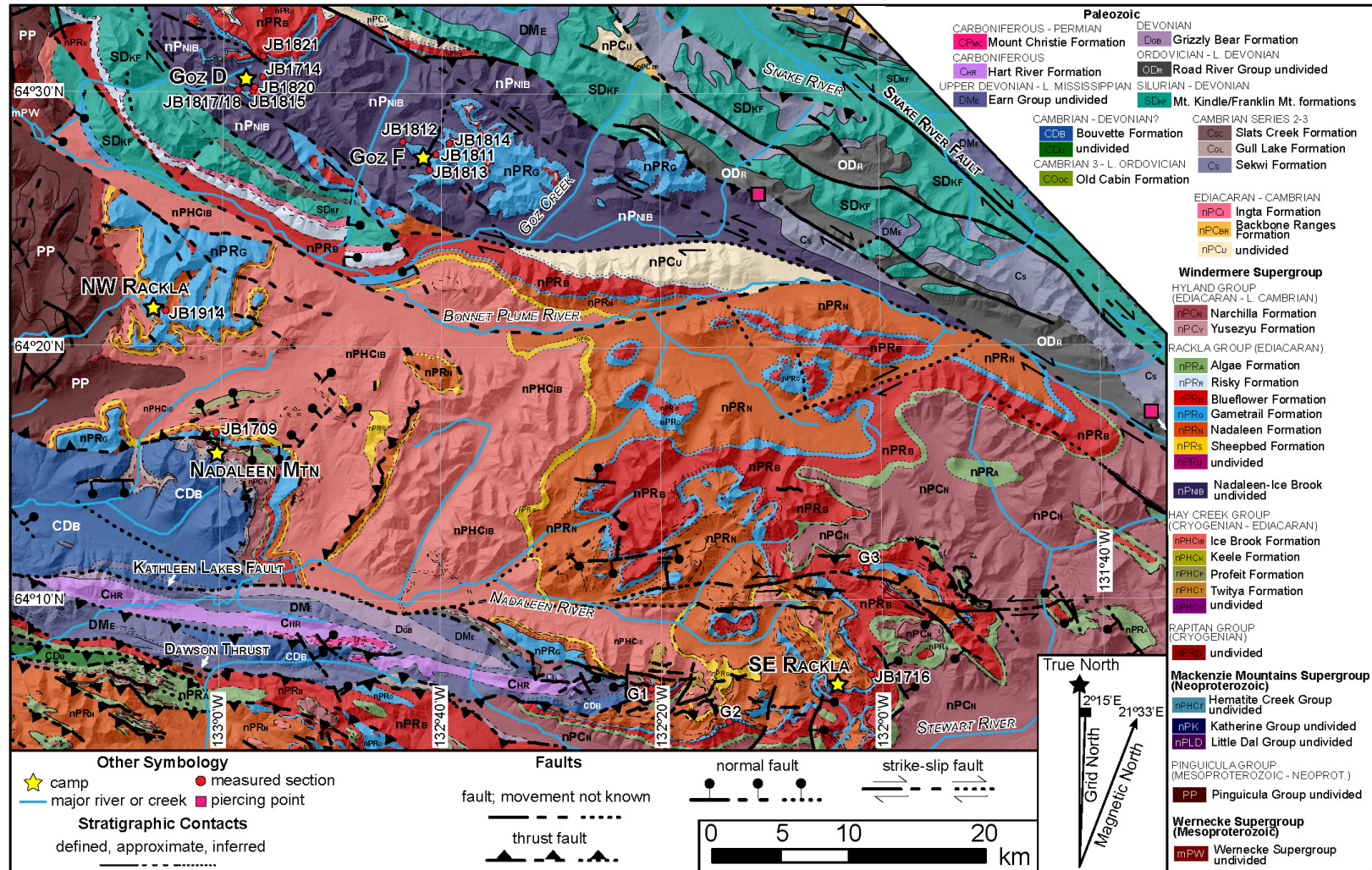
Figure 8. Bedrock geology of the southern Corn/Goze Creek and Nadaleen River regions of the Wernecke Mountains, Yukon. Stratigraphic sections are plotted as red circles and presented in figures 6 and 10. There is an estimated 30 km of dextral displacement along the strike-slip faults which bound the Goz D-F block, with the Sekwi Fm interpreted as a piercing point on displacement (pink squares) for palinspastic restoration. Sections G1, G2, and G3 from Moynihan et al. (2019) are also shown for reference.
