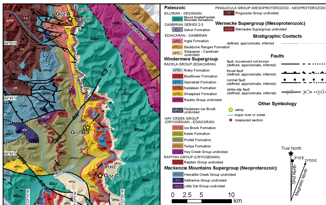
Figure 5. Bedrock geology of the northern Corn/Goat Creek region of the Wernecke Mountains, Yukon. Measured stratigraphic sections are plotted as red circles and presented in figure 6.
