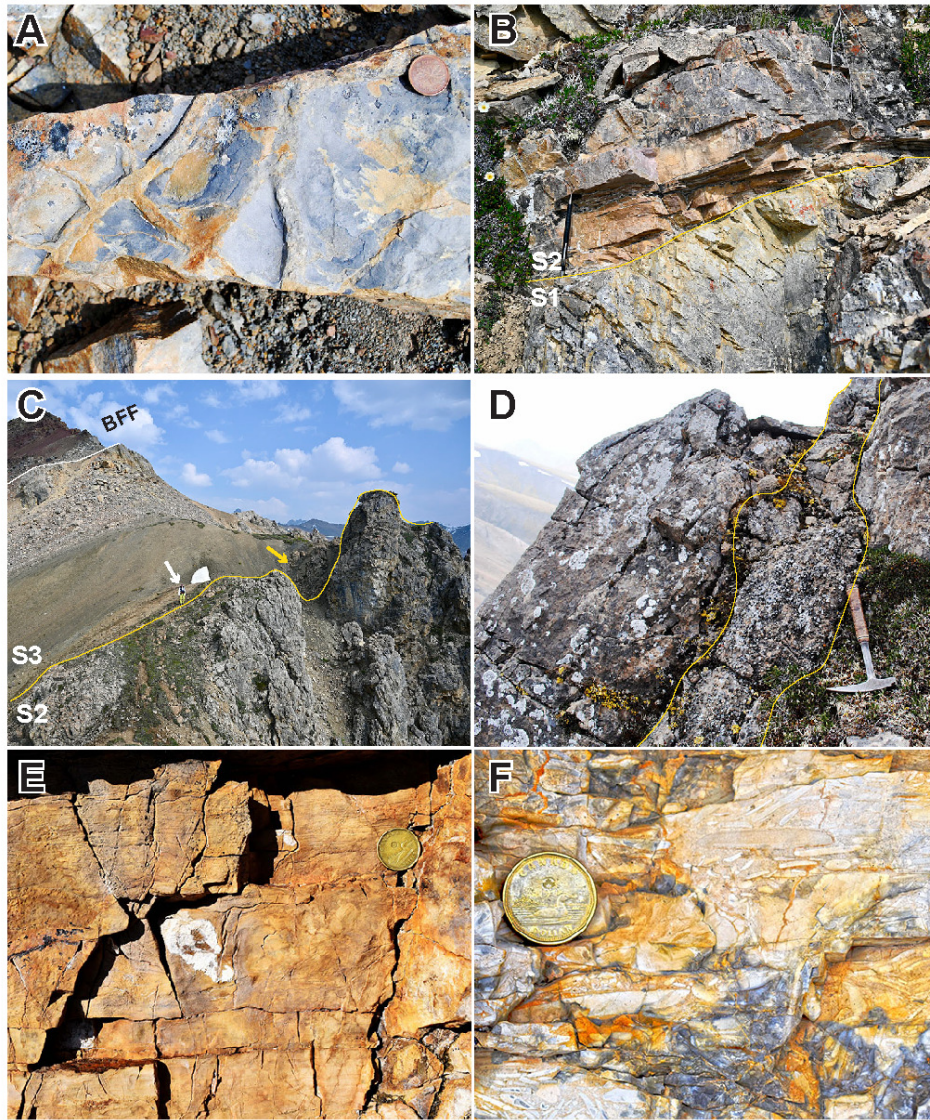
Figure 7. Photo panel of representative lithofacies and stratigraphic relationships from the Gametrail Fm in the northern Corn/Goat Creek region. (A) Mudcracks along a bedding surface of interbedded calcareous siltstone and sandstone at the contact between the Nadaleen and Gametrail formations at Goz A. Coin is 1.9 cm in diameter. (B) Erosional contact (yellow line) between grey stromatolitic doloboundstone (FA3) and tan cross-laminated silty dolograins (FA1) marking the S1-S2 sequence boundary at Goz B. Pencil is 14 cm long. (C) Relict paleokarst topography at the S2-S3 sequence boundary (yellow line) at Goz B. Yellow arrow depicts distinct karst breccia fill and white star outlines geologist for scale; BFF–Blueflower Fm. (D) Paleokarst cavity (outlined in yellow) filled with granule- to cobble-sized clasts of carbonate, chert, and quartzite in a carbonate-cemented quartz sand matrix (FA14) within vuggy recrystallized dolostone (FA10) of the upper Gametrail Fm at Goz A. Rock hammer is 33 cm long. (E) Characteristic tan-orange ripple cross-laminated silty dolograins (FA1) interbedded with microbialite (FA4) in the lower Gametrail Fm at Goz B. Coin is 2.7 cm in diameter. (F) Intraclast rudstone (FA2) composed of tabular pebble/cobble dolograins in a silty dolograins matrix from the lower Gametrail Fm at Goz A. Coin is 2.7 cm in diameter.
