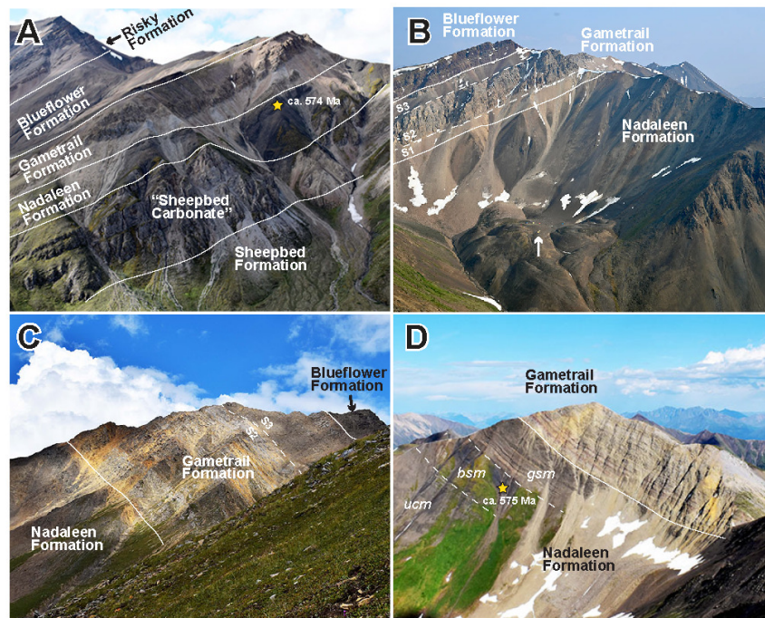
Figure 4. Photographs of selected localities from the northern Corn/Goat Creek and Nadaleen River regions. (A) Image looking southeast at the Rackla Group of Goz A. Yellow star indicates location of Re-Os date shown in figure 2 ; Nadaleen Fm is 87.5 m thick for scale. (B) Image looking southeast at the Rackla Group of Goz B. Note the significant thickness increase and change in outcrop character in the Nadaleen Fm compared to Goz A. Tents are arrowed for scale and the S1-3 depositional sequences are labeled in the Gametrail Fm. (C) Typical outcrop style of the Gametrail Fm in the Nadaleen River area. The S2 and S3 depositional sequences are labeled accordingly in the Gametrail Fm and it is locally ~265 m thick for scale. (D) Image looking east at the Gametrail Fm in the southern Nadaleen River area (Section G2 of Moynihan et al., 2019). Yellow star indicates the interval sampled for Re-Os geochronology ( fig. 2 ) in the black shale member (bsm) of the Nadaleen Fm. Also shown are boundaries between the upper carbonate member (ucm) and green siliciclastic member (gsm) of the Nadaleen Fm.
