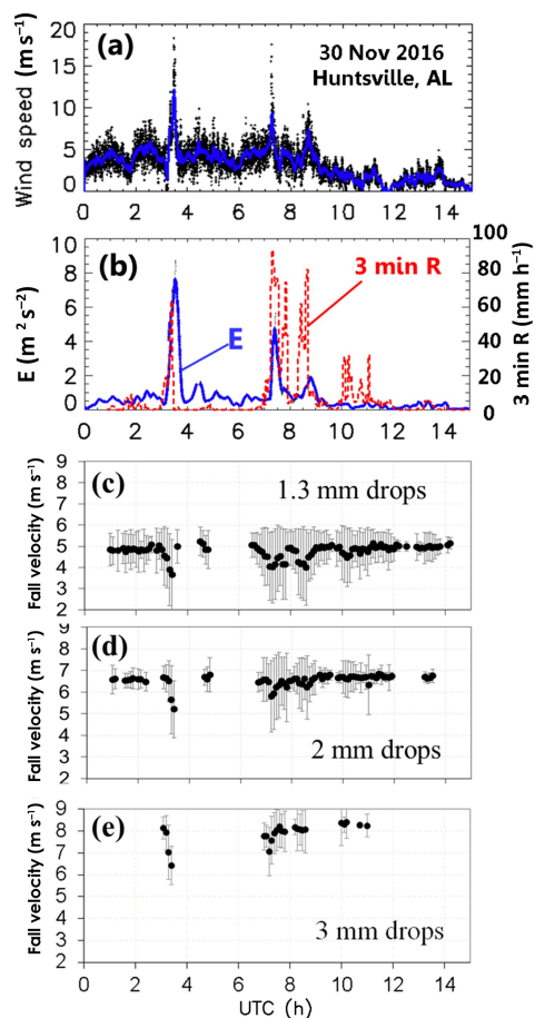
Figure 4. (a) As in Fig. 2a except for 30 November 2016 event. (b) As in Fig. 2b. (c) Mean and 1 SD of fall speeds from 2DVD for 1:30:1 mm sizes. (d, e) As in (c) but for 20:1 and 30:1 mm sizes, respectively.
