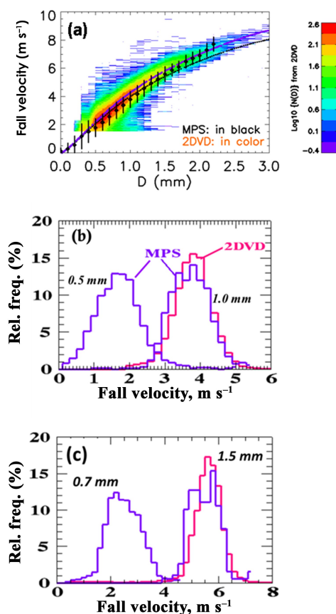
Figure 1. (a) Fall velocity vs. diameter ( D ). The contoured frequency of occurrence from 2DVD data is shown in color (log scale). The mean fall velocity and 1 standard deviation bars are from MPS. The dark dashed line is from the fit to the laboratory data of Gunn and Kinzer (1949) and the purple line is the same except corrected for the altitude of Greeley, CO (1.4 km m.s.l.). (b) Relative frequency histograms of fall velocity for the 0:50:1 mm and 10:1 mm bins. (c) As in (b) but for the 0:70:1 mm and 1:50:1 mm bins.
