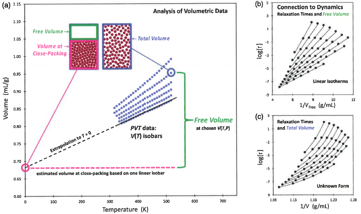
FIG. 1. (a) PVT data for a polyvinylacetate melt [35] plotted in the form of V(T) isobars at P = 0, 40, 80, 120, 160 , and 200 MPa, and diagrams depicting how to define and estimate free volume, V_{\text{free}}(T, P) [Eq. (2)]. (b) T, P dependent segmental relaxation times [36] correlated against V_{\text{free}}(T, P) estimated via the method in panel (a); plot shows \log \tau(T, P) vs 1/V_{\text{free}}(T, P) on isotherms of varied T (333 to 413 K). (c) Same relaxation times correlated against total volume, \log \tau(T, P) vs 1/V(T, P) .
