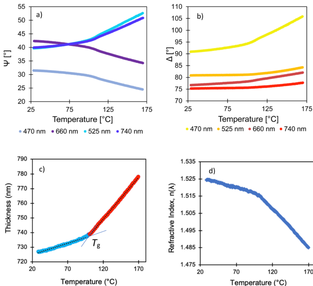
Fig. 2 (a) Ellipsometric data obtained from a dynamic heating scan for a thin film of PCHMA using four wavelengths as are shown in the legend: (a) data and (b) \Delta data. (c) Thickness of this film as a function of temperature, obtained from the analysis of the data shown in (a) and (b). The \alpha_N value in the temperature range from 28 to 101 °C (attributed to the glass region) is 2.12 (\pm 0.02) \times 10^{-4} \text{ °C}^{-1} , whereas in the temperature range from 105 to 170 °C (attributed to the melt region) \alpha_N = 7.52 (\pm 0.02) \times 10^{-4} \text{ °C}^{-1} . The glass transition temperature is indicated by the change in the gradient. (d) Refractive index, n (at a wavelength of 0.55 \mu\text{m} ) as a function of temperature for the same film.
