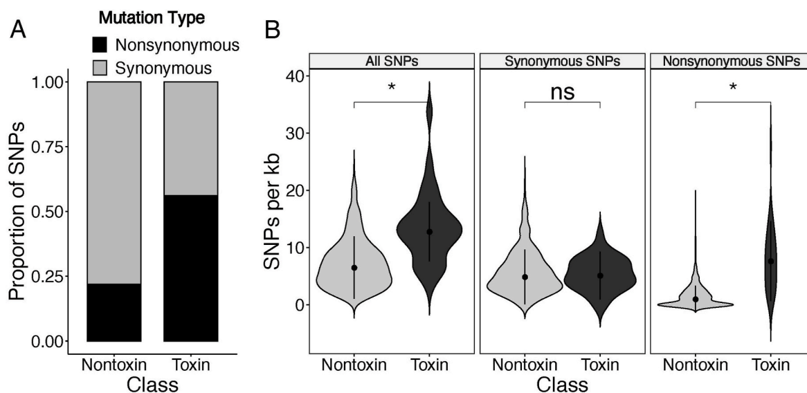
Fig. 3. The number and type of SNPs found in toxin and nontoxin transcripts. (A) Toxins maintain a higher ratio of nonsynonymous to synonymous SNPs. (B) Toxins have a higher number of SNPs per kilobase (kb) with nonsynonymous SNPs driving this difference (*: significant; ns: not significant).
