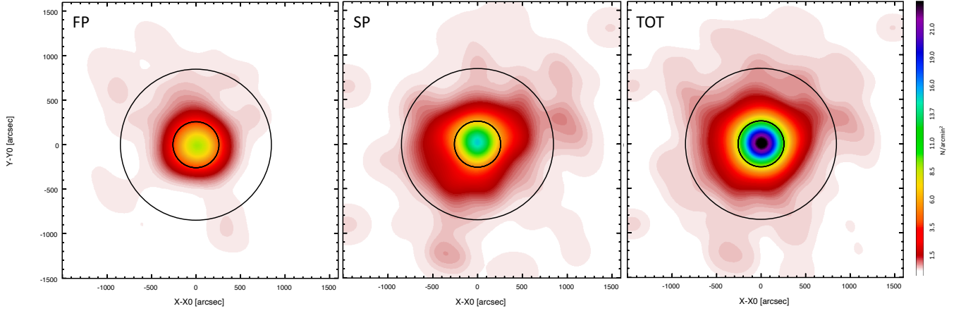
Fig. 6. Color-coded surface density map of the analyzed field of view centered on the position of NGC 3201. The left panel shows the 2D map of the FP, the central panel that of SP stars and right panel the 2D map of total population (i.e., SP+FP). The inner and outer circles in each panel have a radius of 250'' and 800'', respectively. North is up, east is right.
