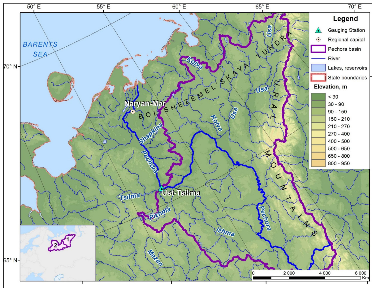
Figure 1. Schematic map of the Pechora River Basin showing the location of Ust'-Tsil'ma Village. In insert: Pechora (1) and Northern Dvina (2) River Basins.
