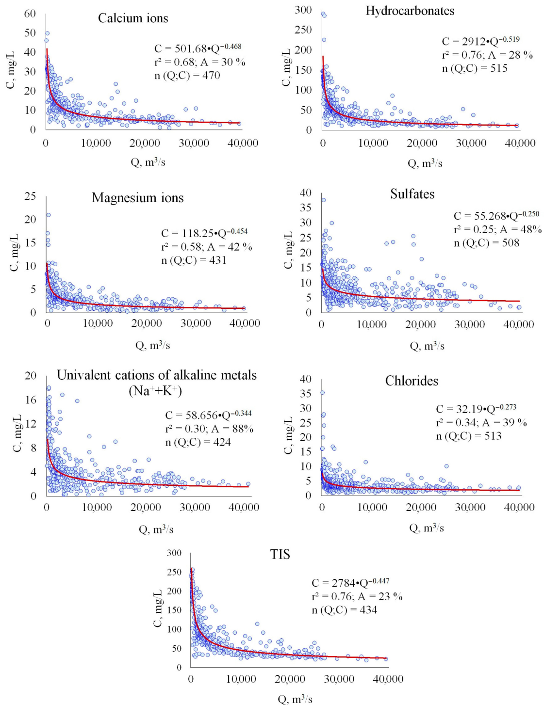
Figure 2. Relationships between major ion concentrations, TIS (C, mg/L) and daily water flow rate (Q, m³/s) for the Pechora River at Ust'-Tsil'ma Village hydrometric station.
