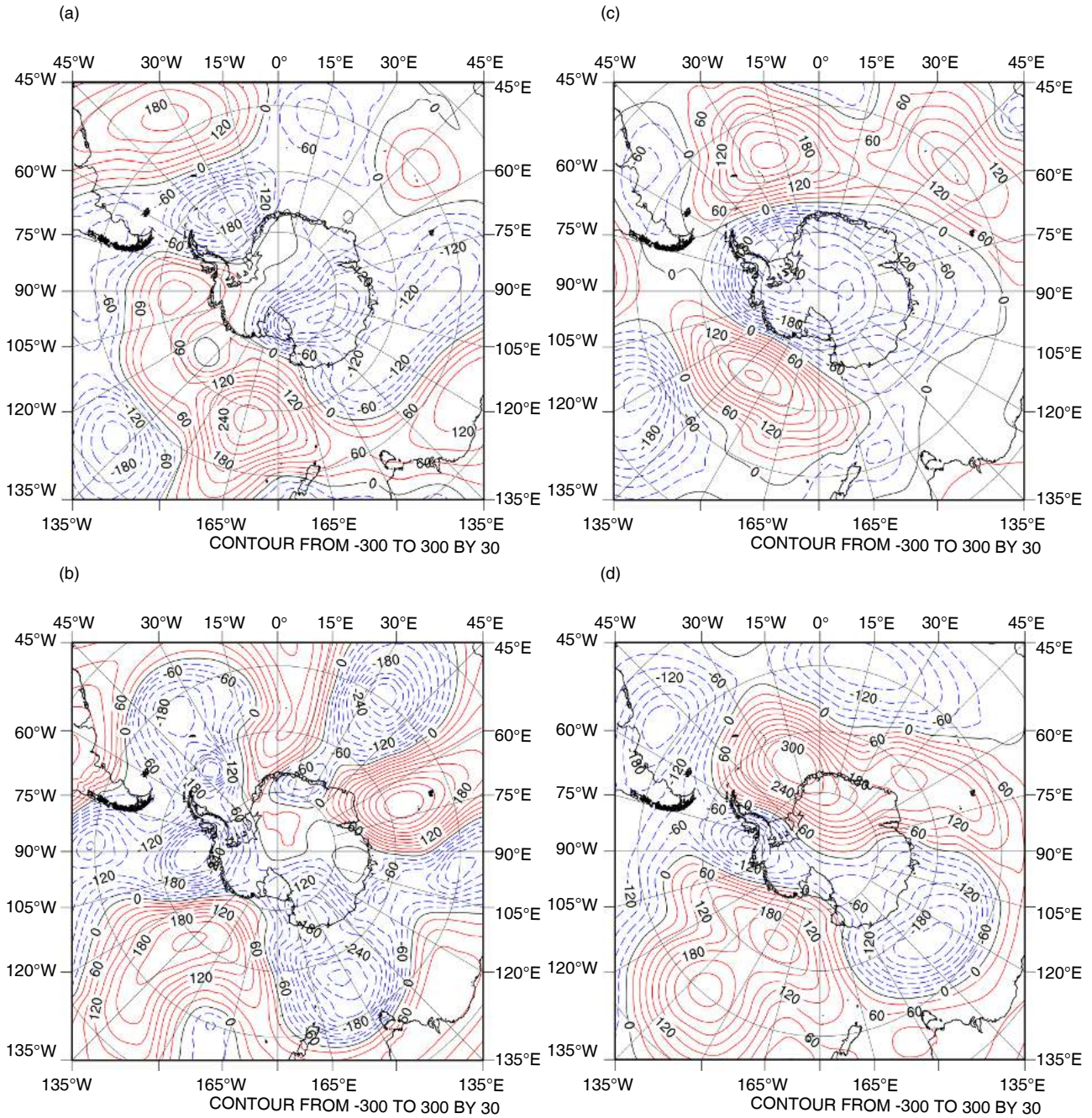
Fig. 4. ERA5 500-hPa anomalies during the four main cold phases contoured every 30 m from -300 to 300 m for (a) 21–23 July, (b) 31 July–1 August, (c) 10–13 August, and (d) 19–24 August.
