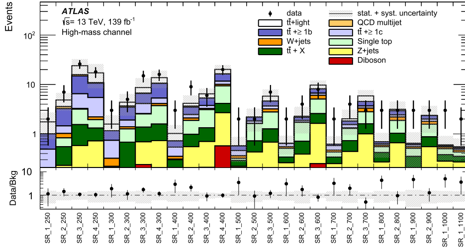
FIG. 9. Postfit SR yields in the high-mass channel. The upper panel shows the observed number of events, as well as the postfit background predictions in each region. The bottom panel shows the ratio of the observed data to the total background prediction. The shaded areas correspond to the total statistical and systematic uncertainties obtained after the fit and described in Sec. VI.
