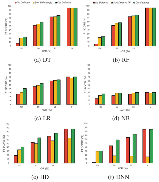
Fig. 7: F_1 Score Comparison Among No Defense , SoA Defense (AT) [8], and Our Defense (ROLDEF)
