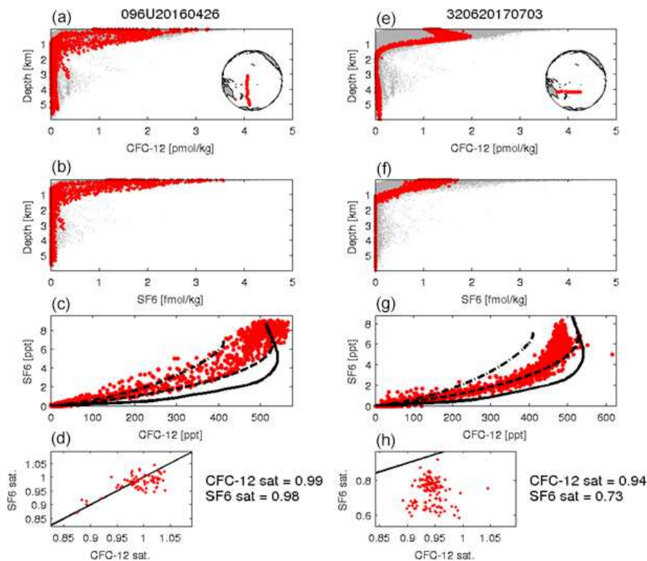
Figure 6. Example of plots used as basis for the SF 6 QC procedure. Shown are the results for cruises 096U20160426 (left) and 320620170703 (right). (a, e) CFC-12 versus pressure for the specific cruise (red), together with all data from the corresponding GLODAP region (Pacific in this case; gray). (b, f) Same as the upper row but for SF 6 . (c, g) CFC-12 versus SF 6 (red dots). Here the measured contents have been converted into atmospheric mixing ratios. Solid black lines show the atmospheric time history of CFC-12 versus that of SF 6 . Dotted lines show CFC-12 versus SF 6 derived from the TTD method for two different sets of TTD parameters. (d, h) CFC-12 vs. SF 6 saturation for the surface layer ( P < 20 dbar), where the numbers give the mean saturation.
