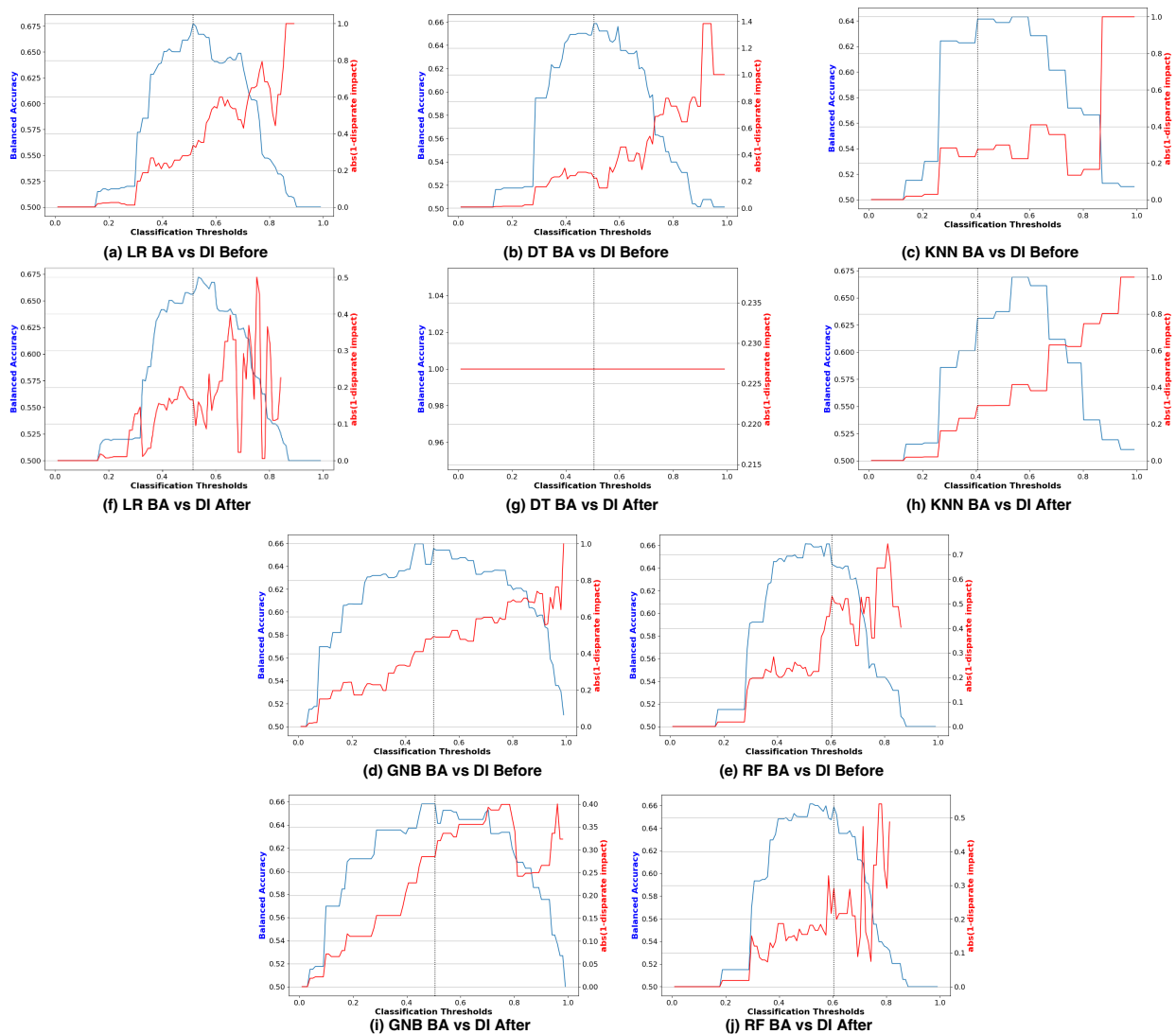
Figure 8. Performance comparison via BA vs. DI before and after reweighting samples on COMPAS dataset with respect to the protected attribute Sex .
