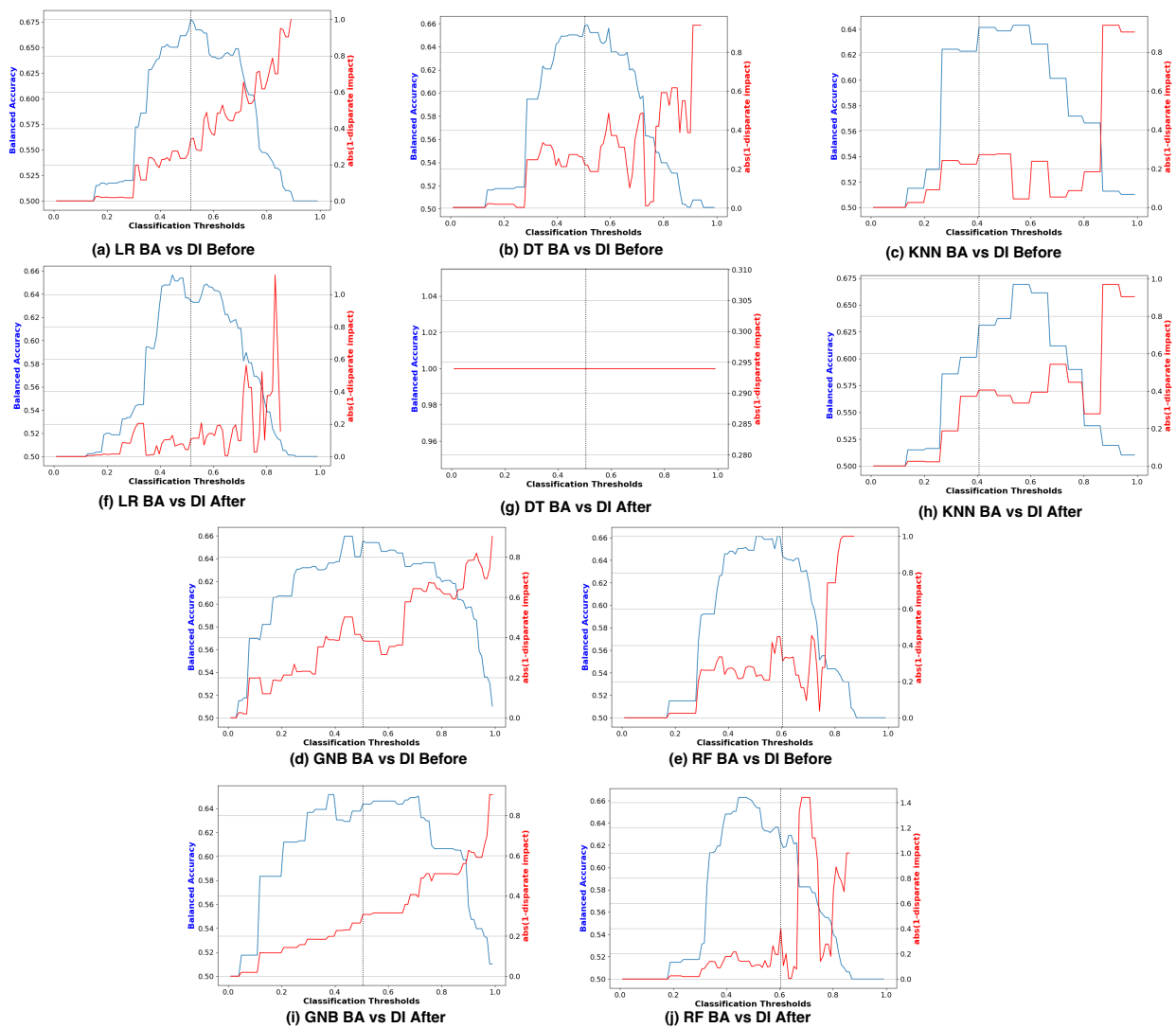
Figure 6. Performance comparison via BA vs. DI before and after reweighting samples on COMPAS dataset with respect to the protected attribute Race .
