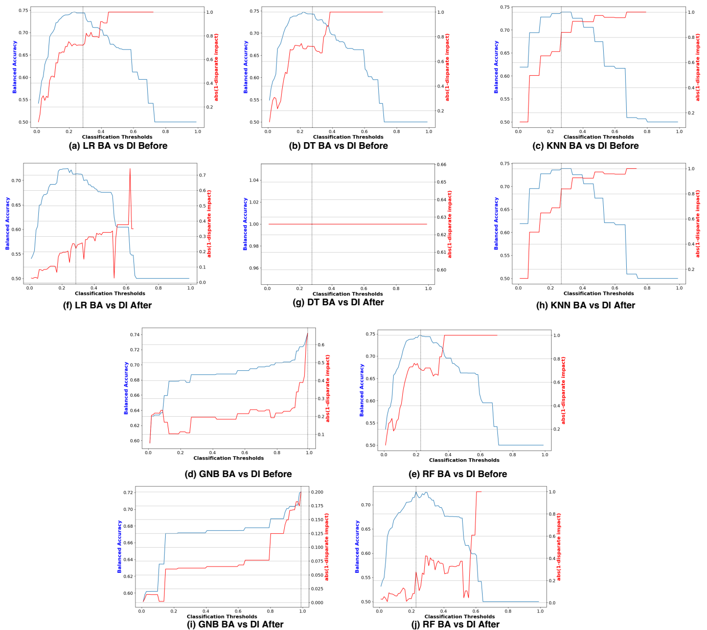
Figure 4. Performance comparison via BA vs. DI before and after reweighting samples on Adult Income dataset with respect to the protected attribute Sex .
