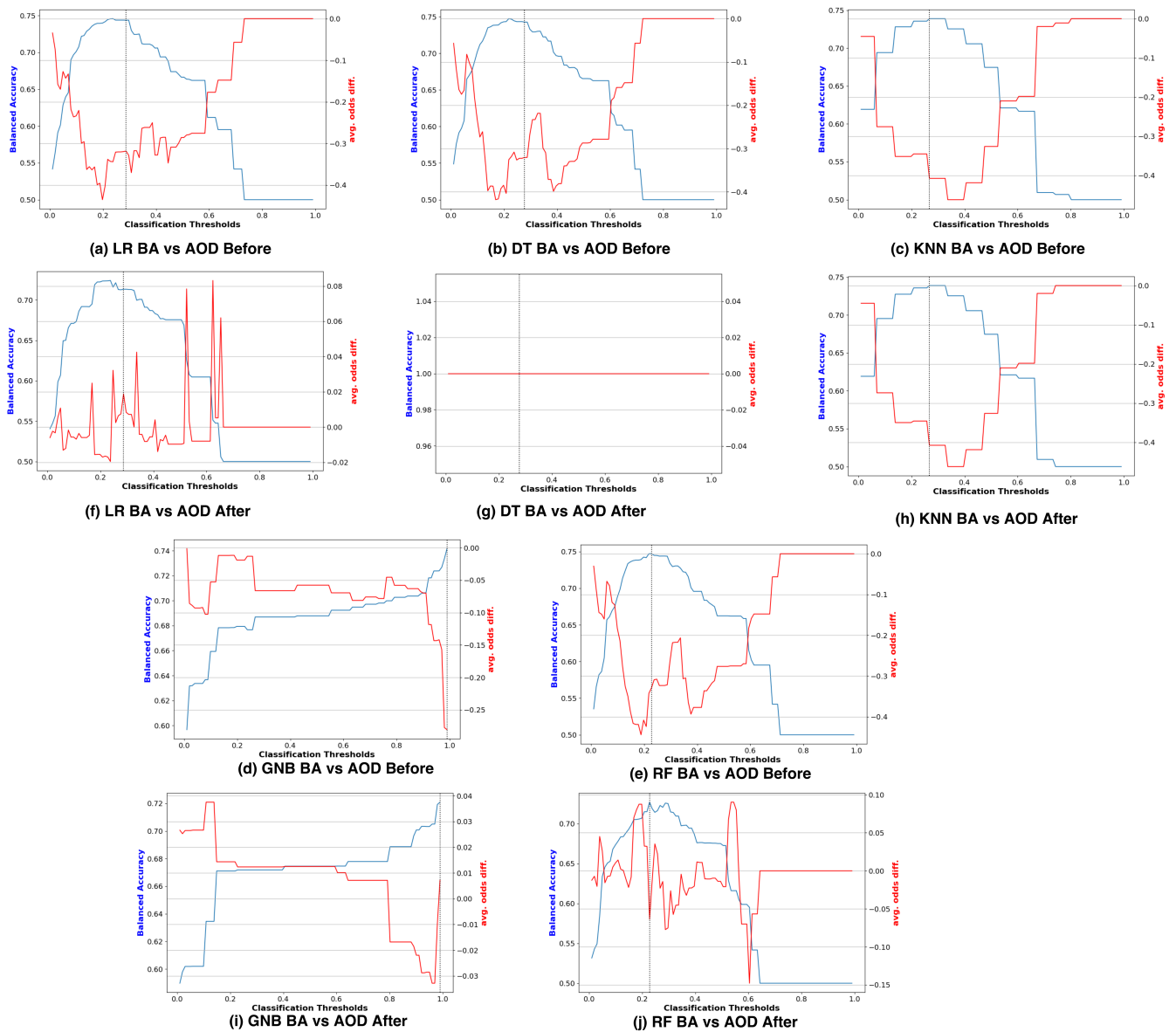
Figure 3. Performance comparison via BA vs. AOD before and after reweighting samples on Adult Income dataset with respect to the protected attribute Sex .
