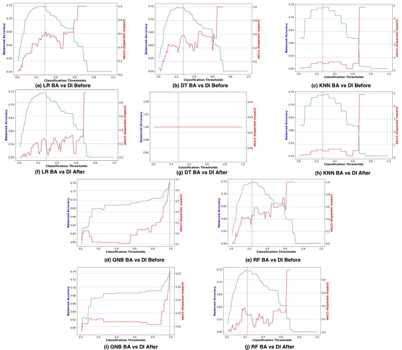
Figure 2. Performance comparison via BA vs. DI before and after reweighting samples on Adult Income dataset with respect to the protected attribute Race .
