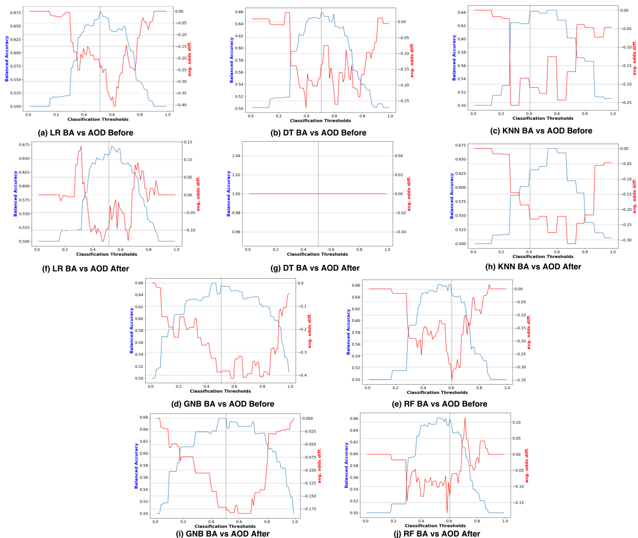
Figure 7. Performance comparison via BA vs. AOD before and after reweighting samples on COMPAS dataset with respect to the protected attribute Sex .
