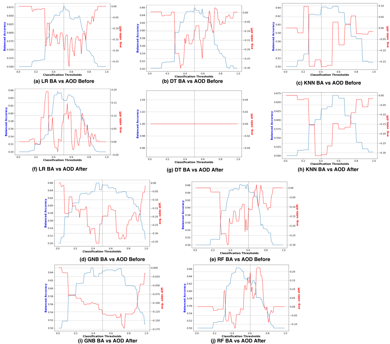
Figure 5. Performance comparison via BA vs. AOD before and after reweighting samples on COMPAS dataset with respect to the protected attribute Race .
