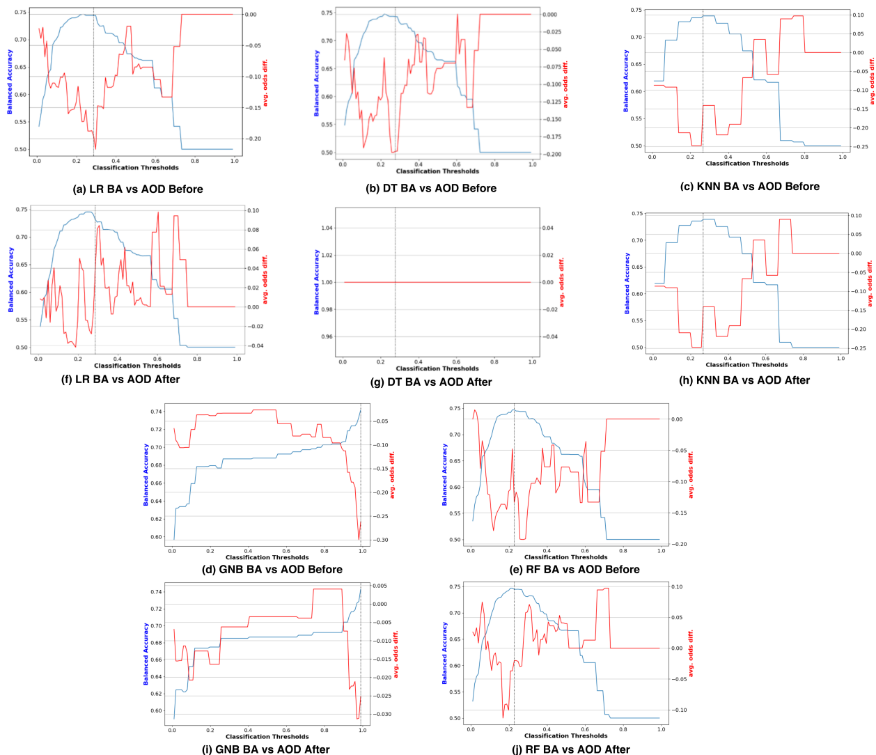
Figure 1. Performance comparison via BA vs. AOD before and after reweighting samples on Adult Income dataset with respect to the protected attribute Race .
