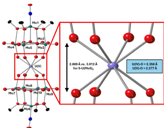
Fig. 10 Single crystal X-ray diffraction structure of 6\text{-U}(\text{Mo}_5)_2 with probability ellipsoids set at 50%. The tetrabutylammonium cation and some disorder has been masked for clarity. Detailed bond length data is given in the ESI.†
